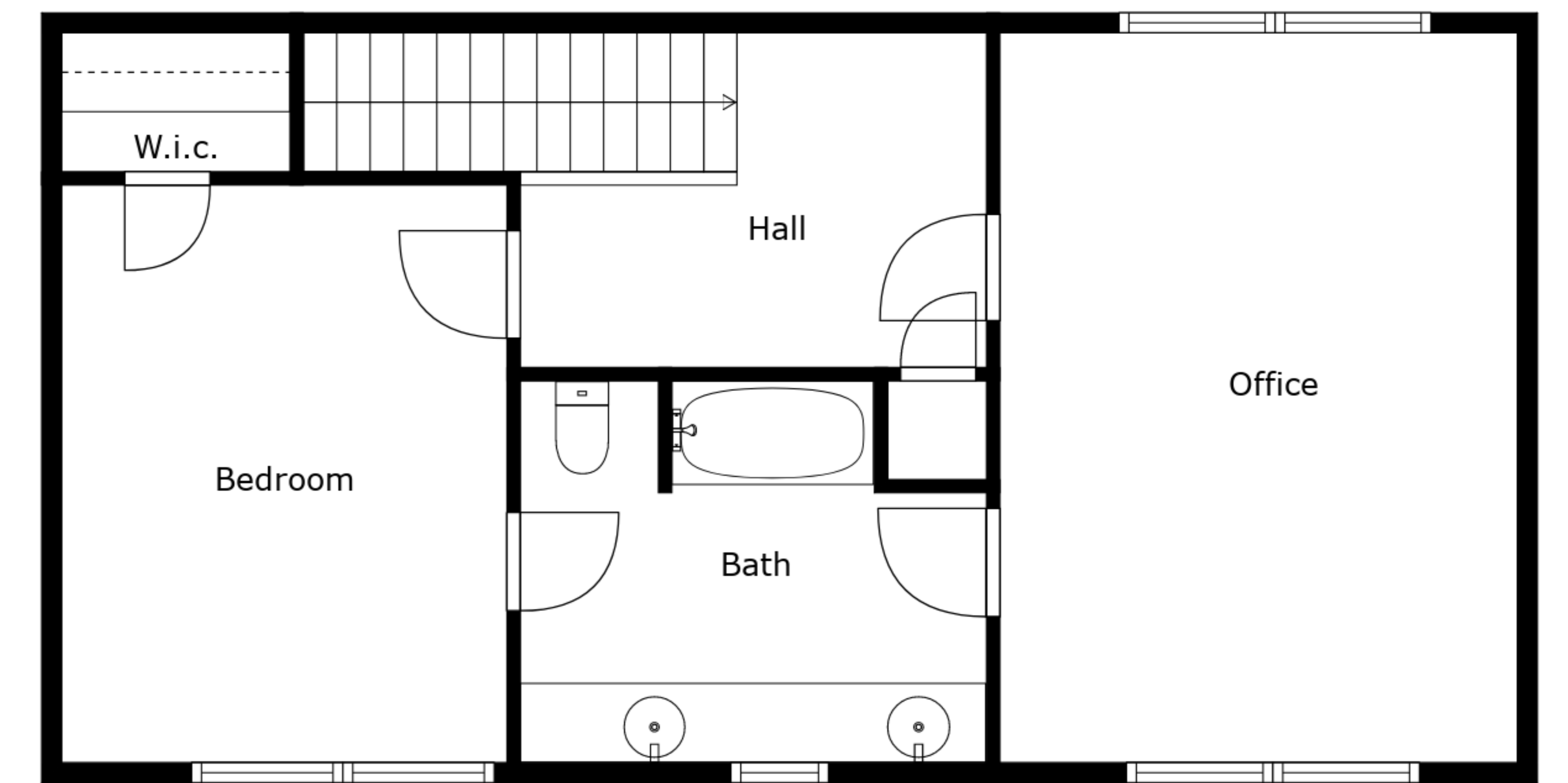
Floor 2
