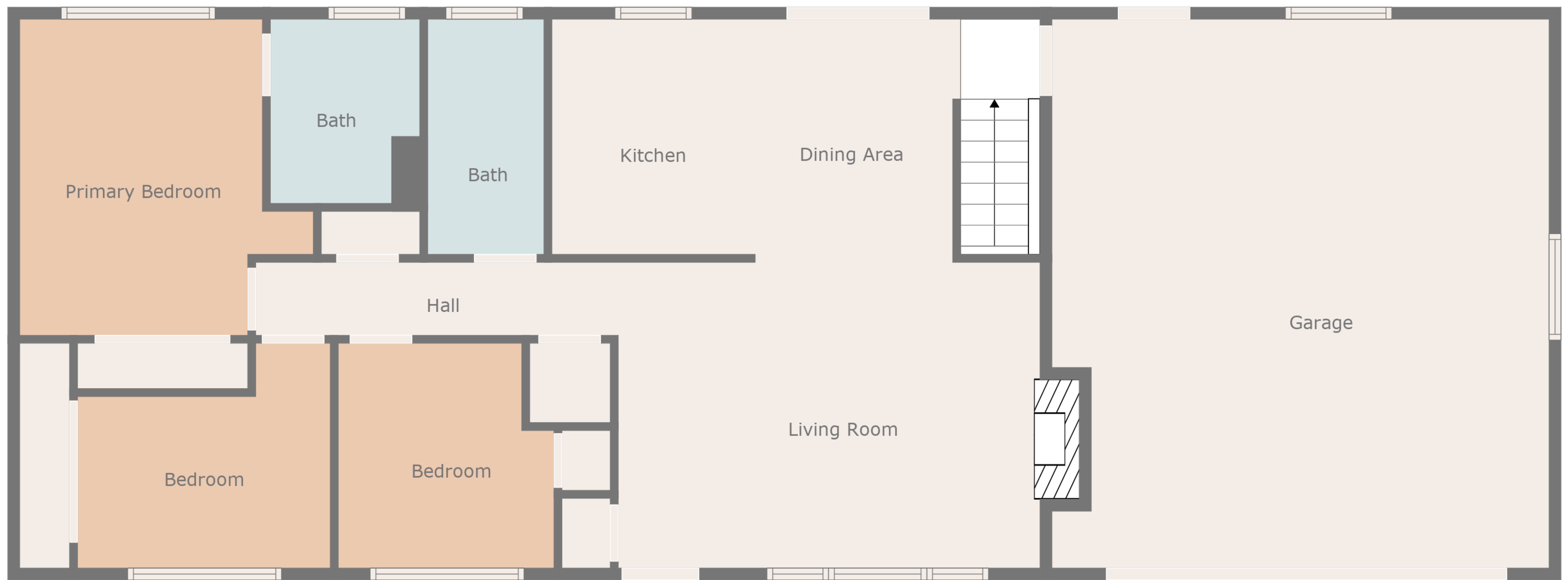
Floor 2
