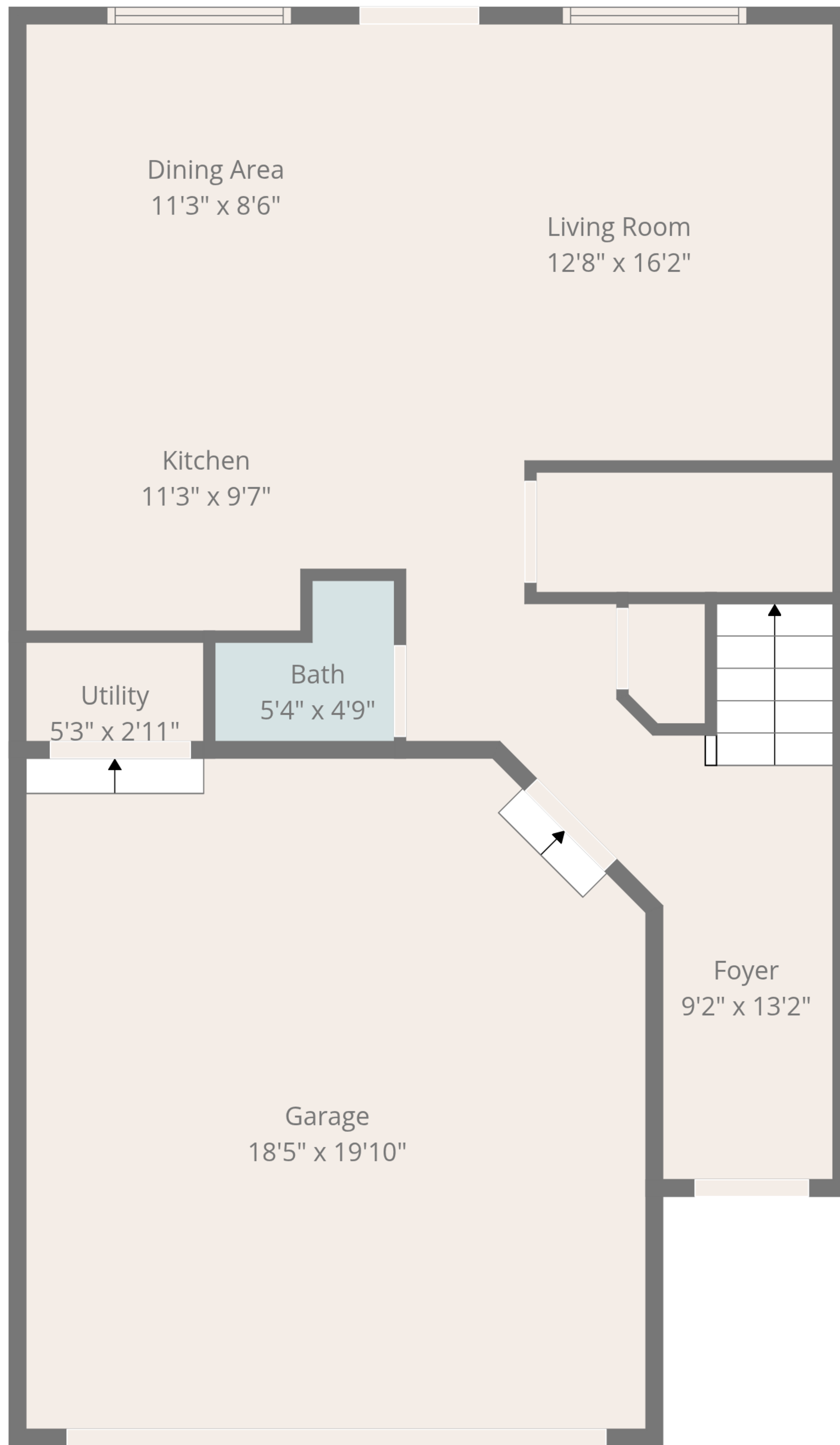
1st Floor
