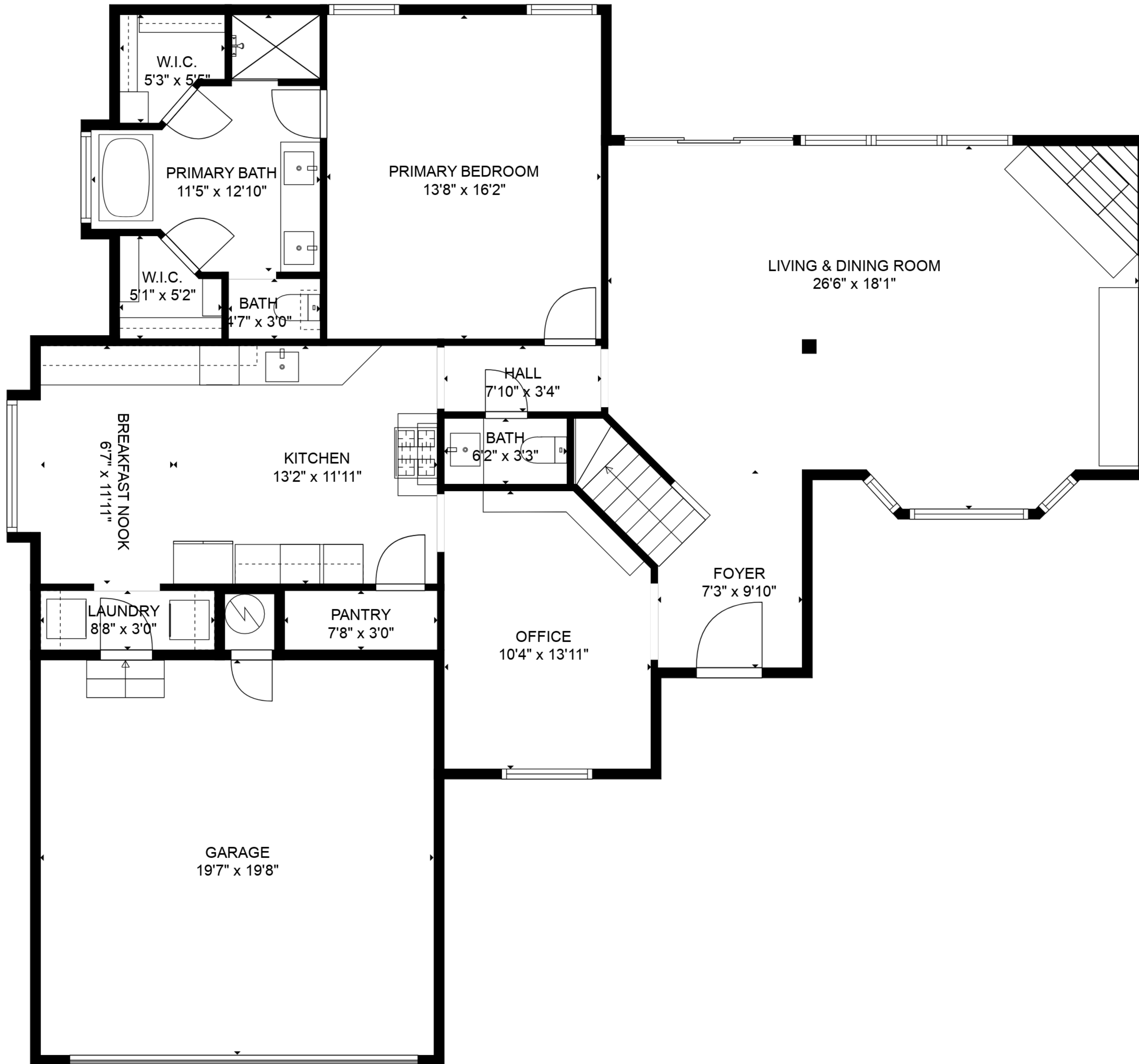
FLOOR 1
