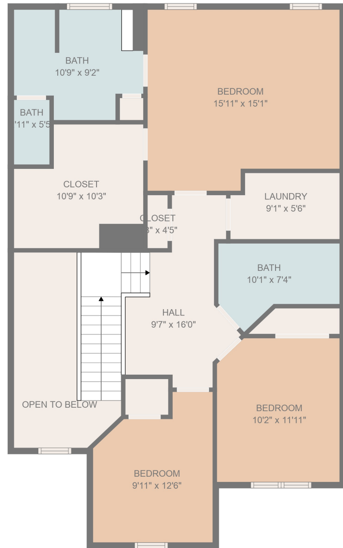
FLOOR 2
