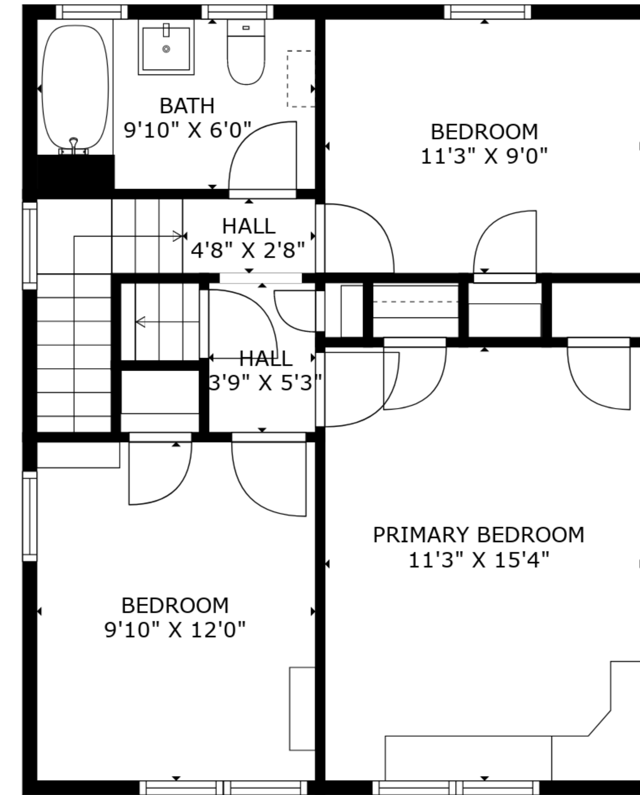
SECOND FLOOR
