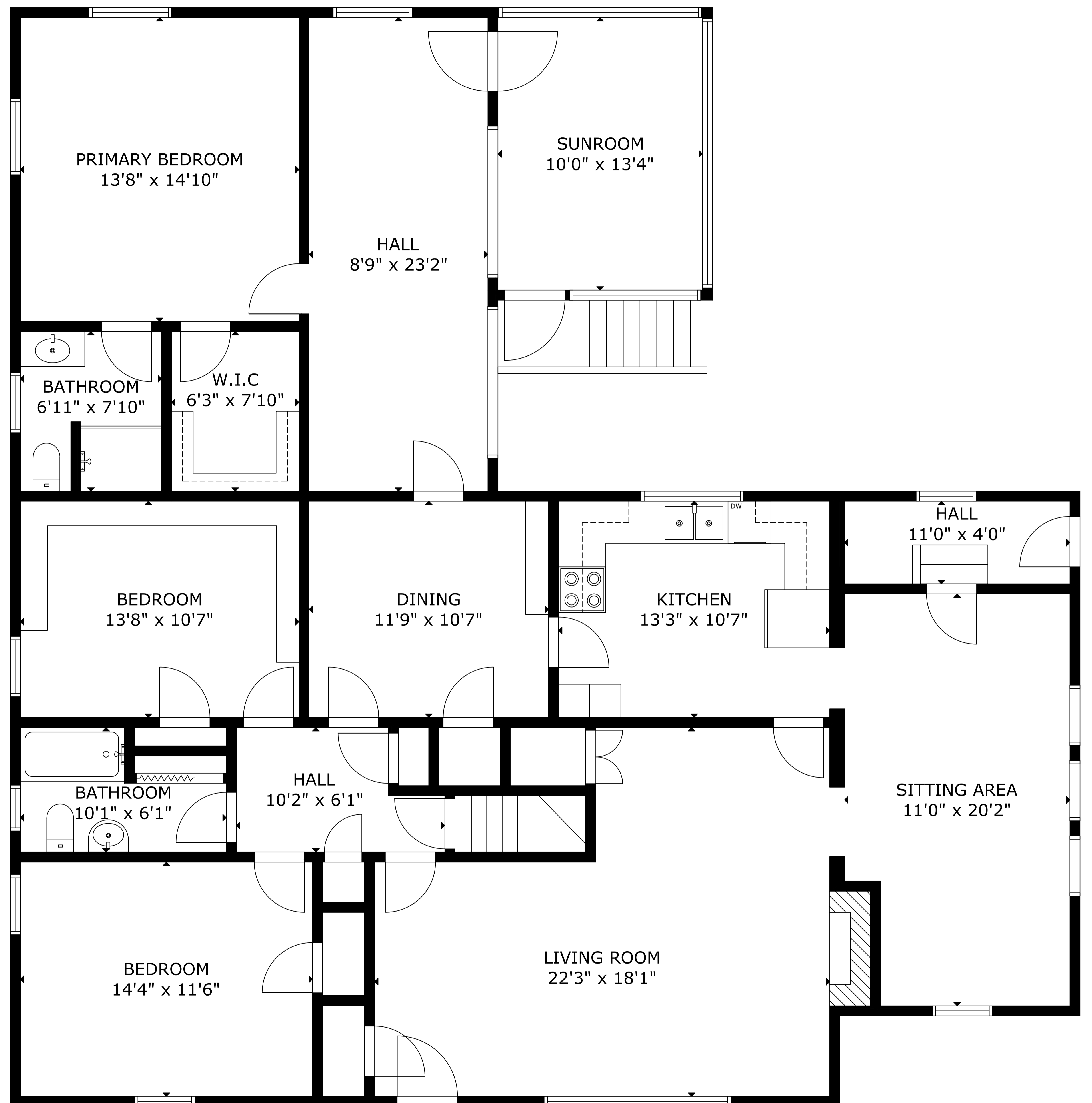
MAIN FLOOR
