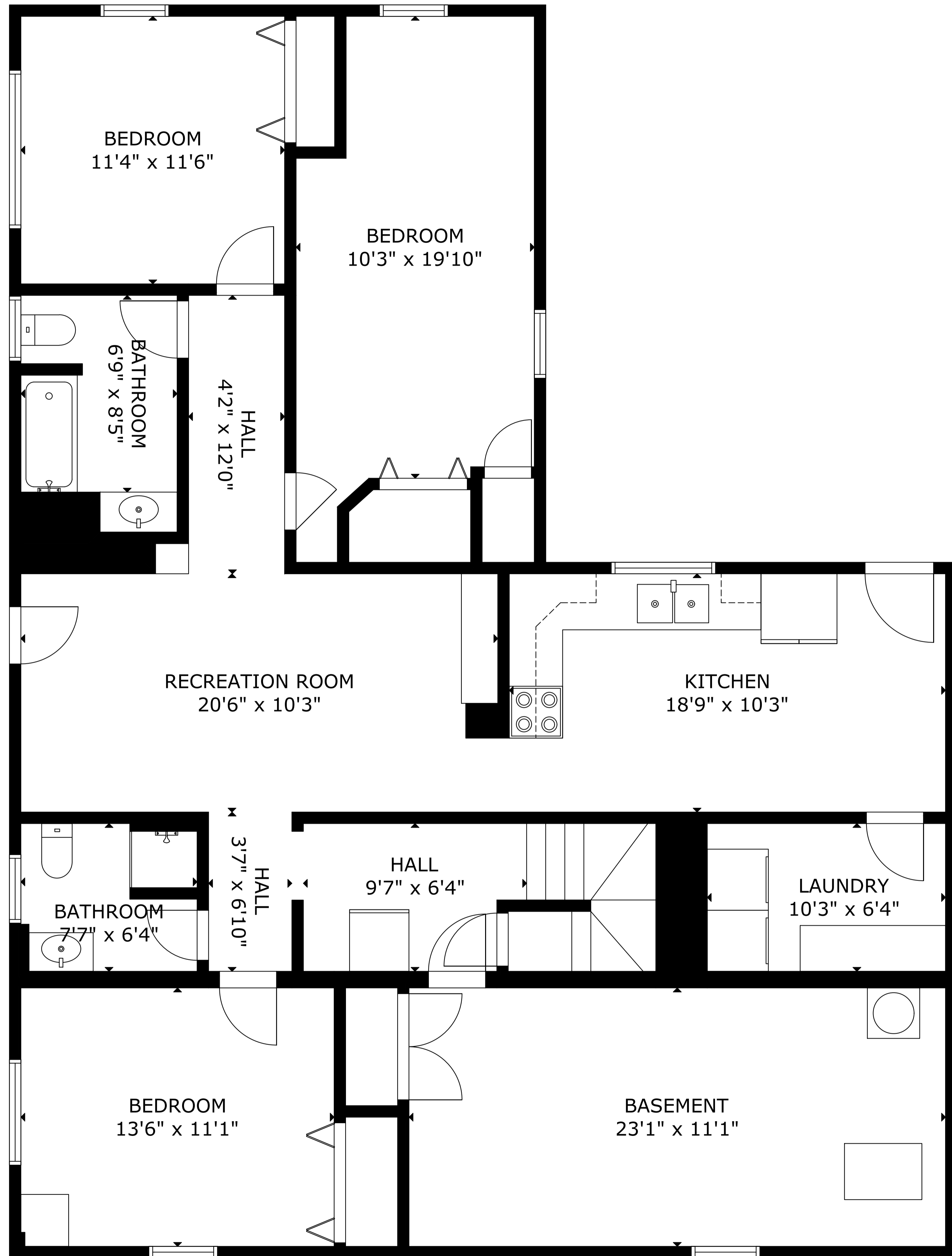
LOWER FLOOR
