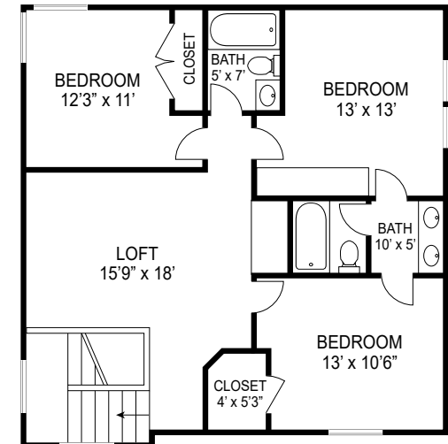
SECOND FLOOR 883 sqf
