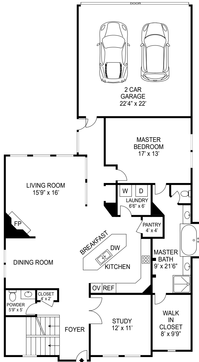
FIRST FLOOR 1647 sqf
