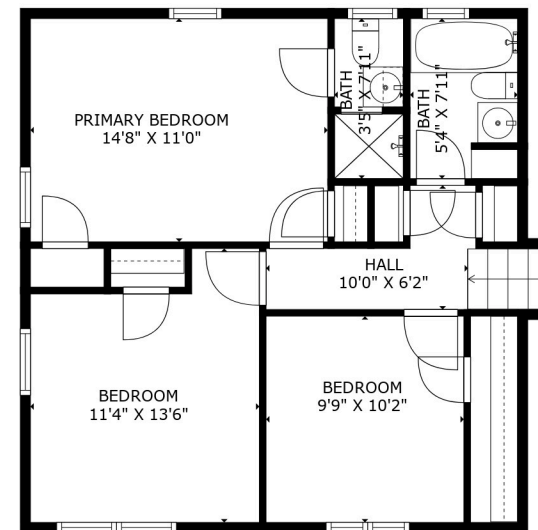
FLOOR 3
