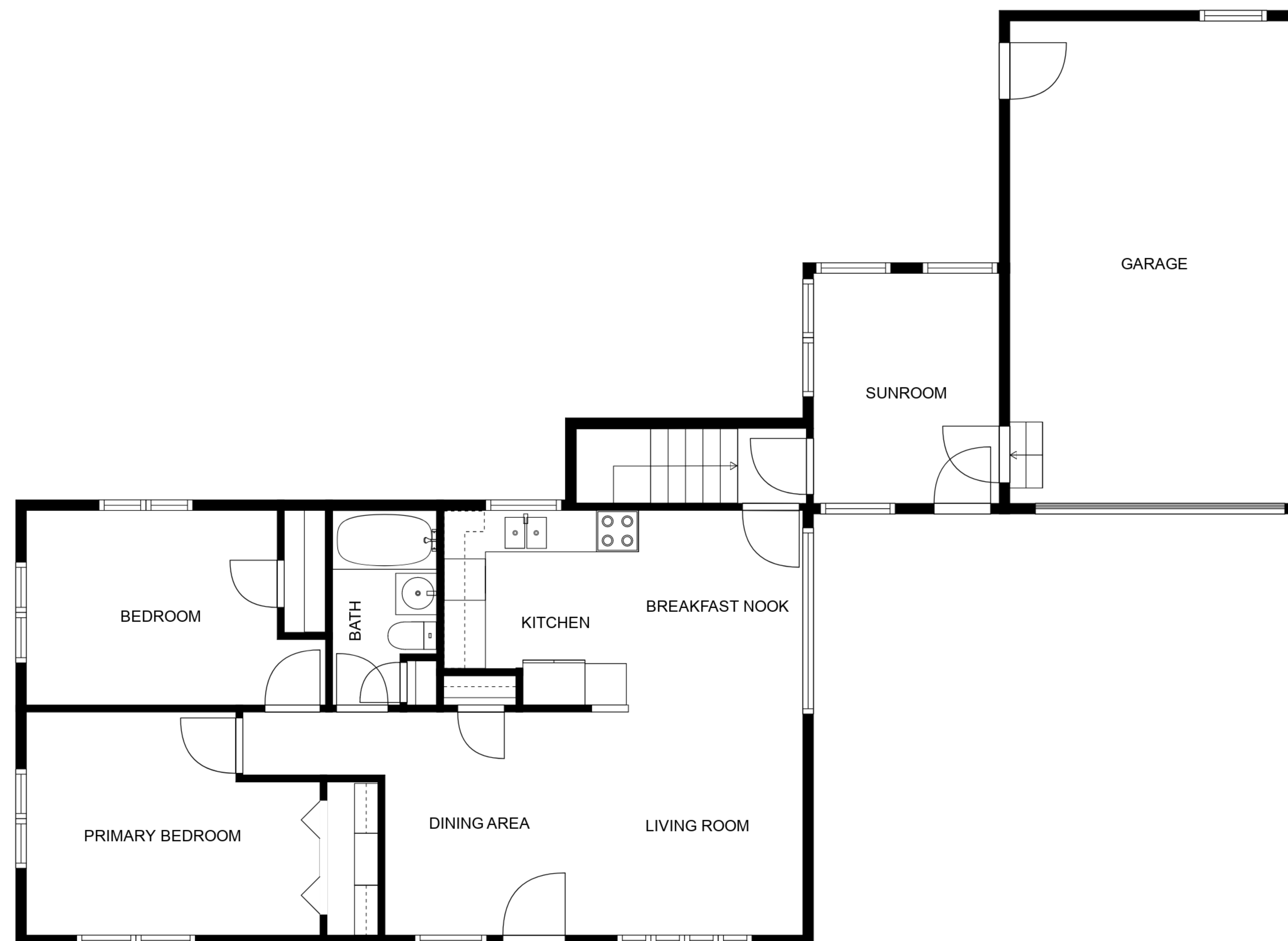
FLOOR 2
