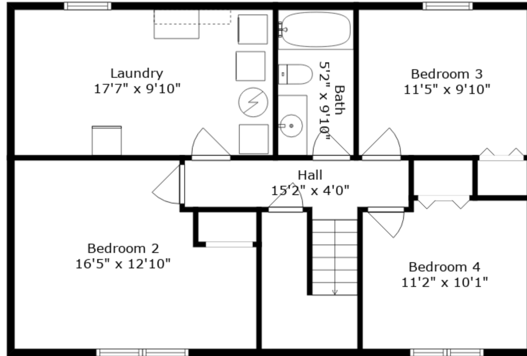
Main Floor
