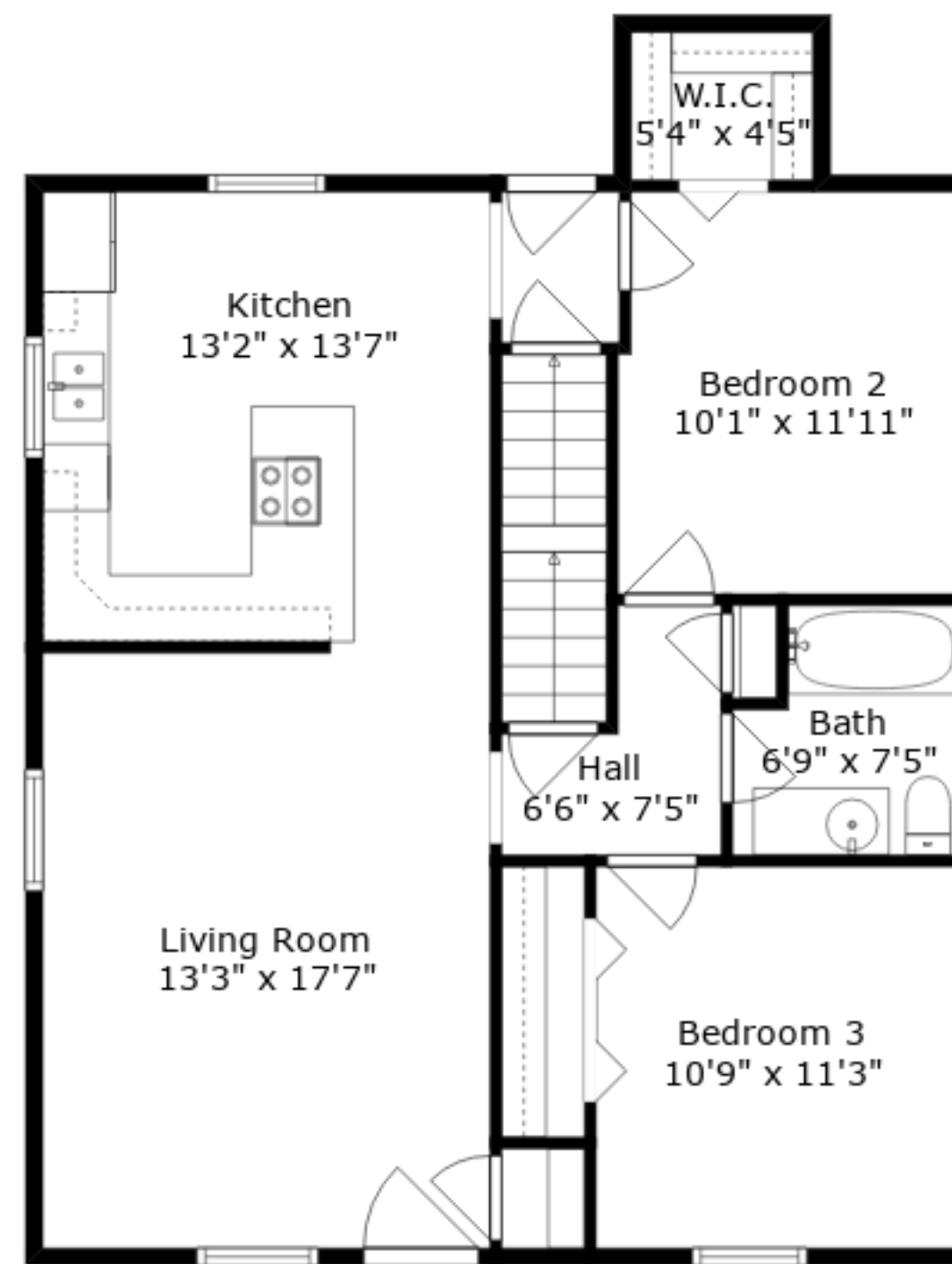
Main Floor
