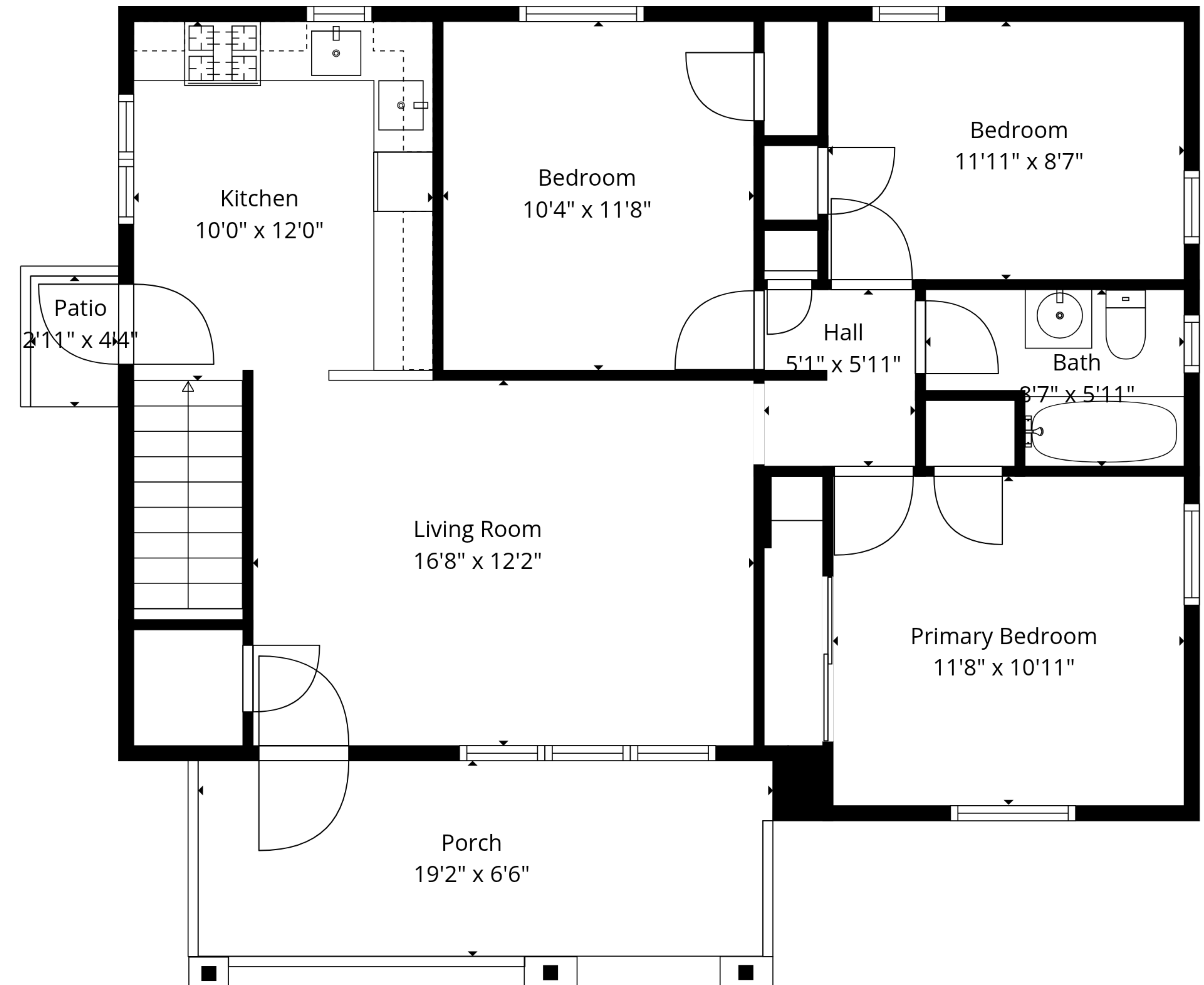
Floor 2
