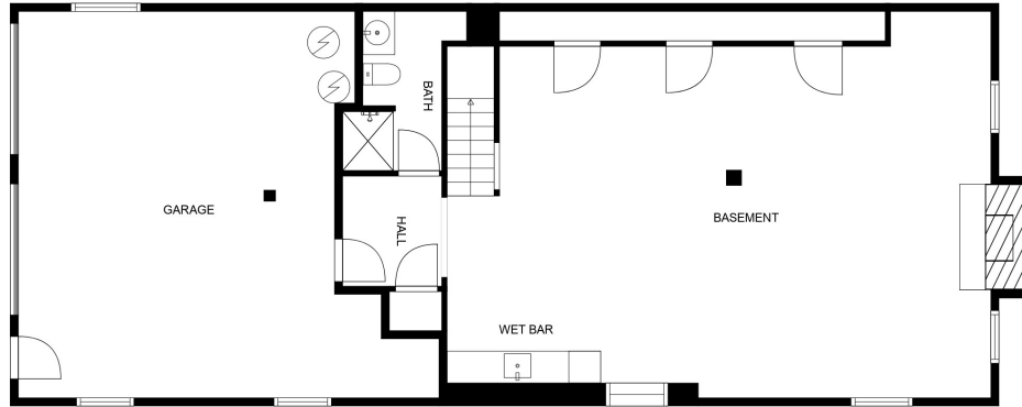
FLOOR 1
