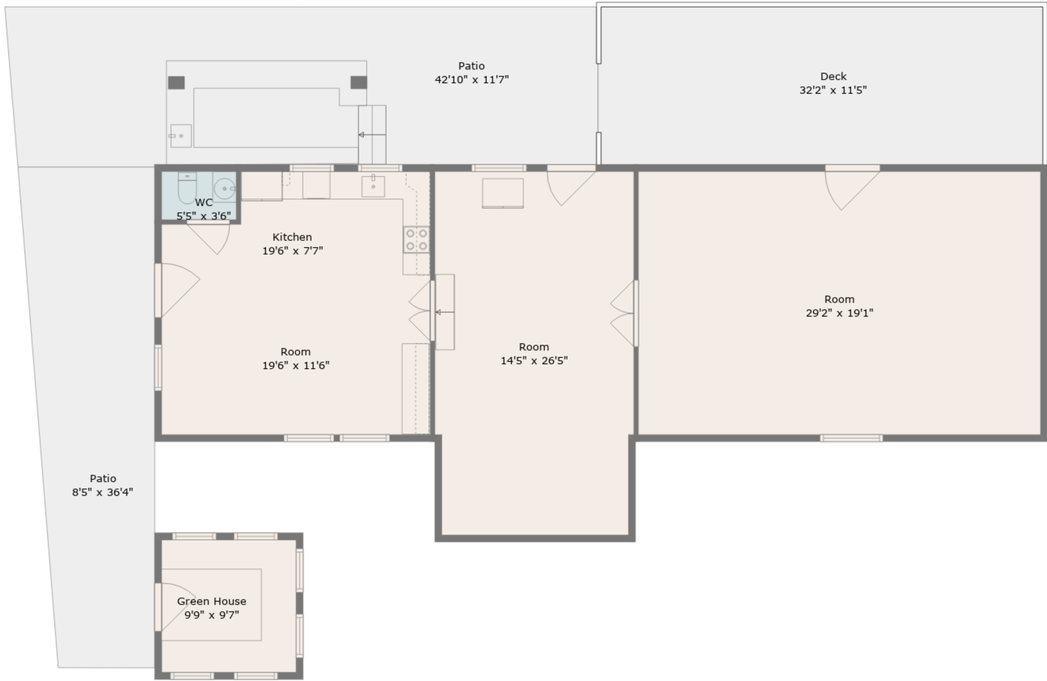
Floor 1
