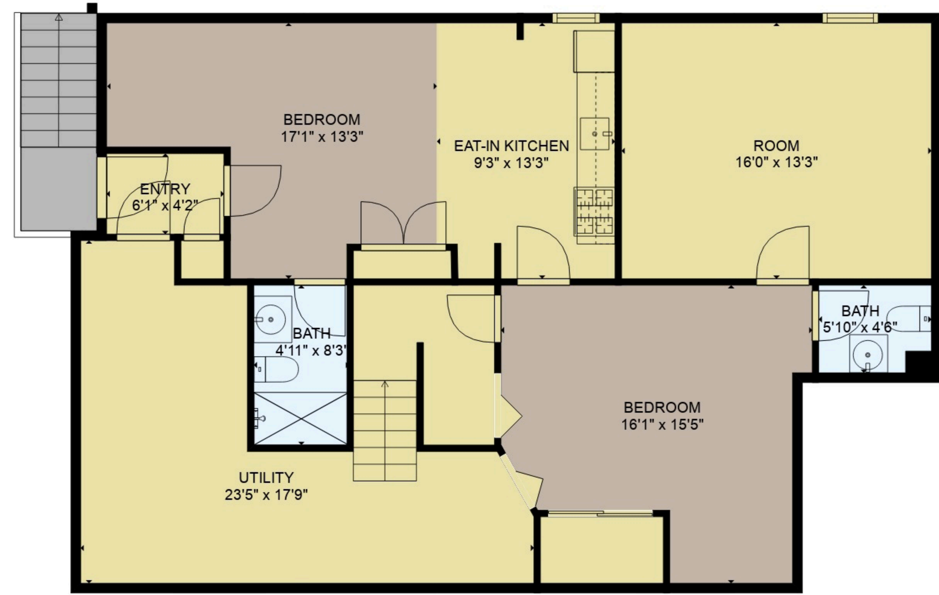
FLOOR 1
