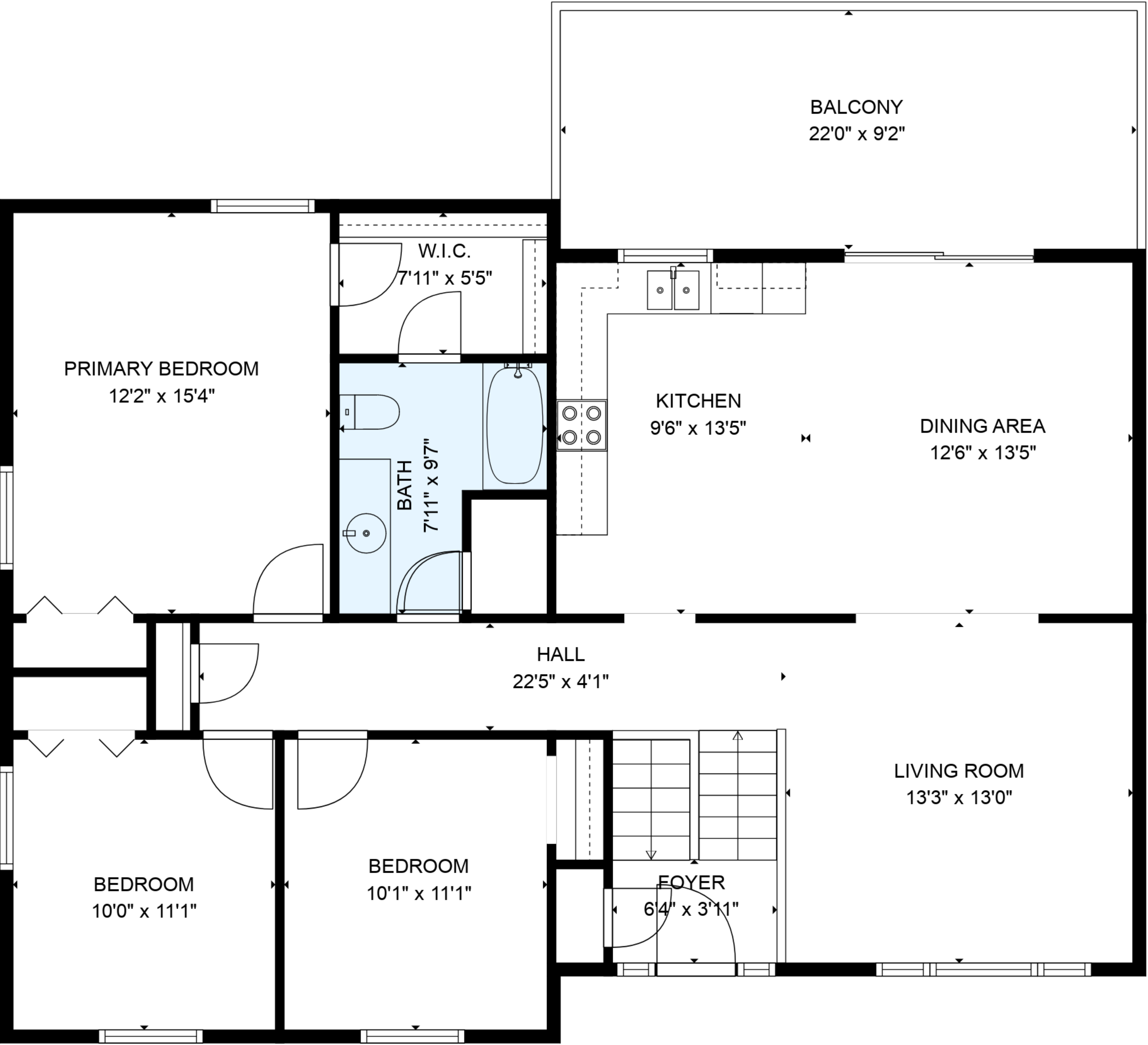
FLOOR 2
