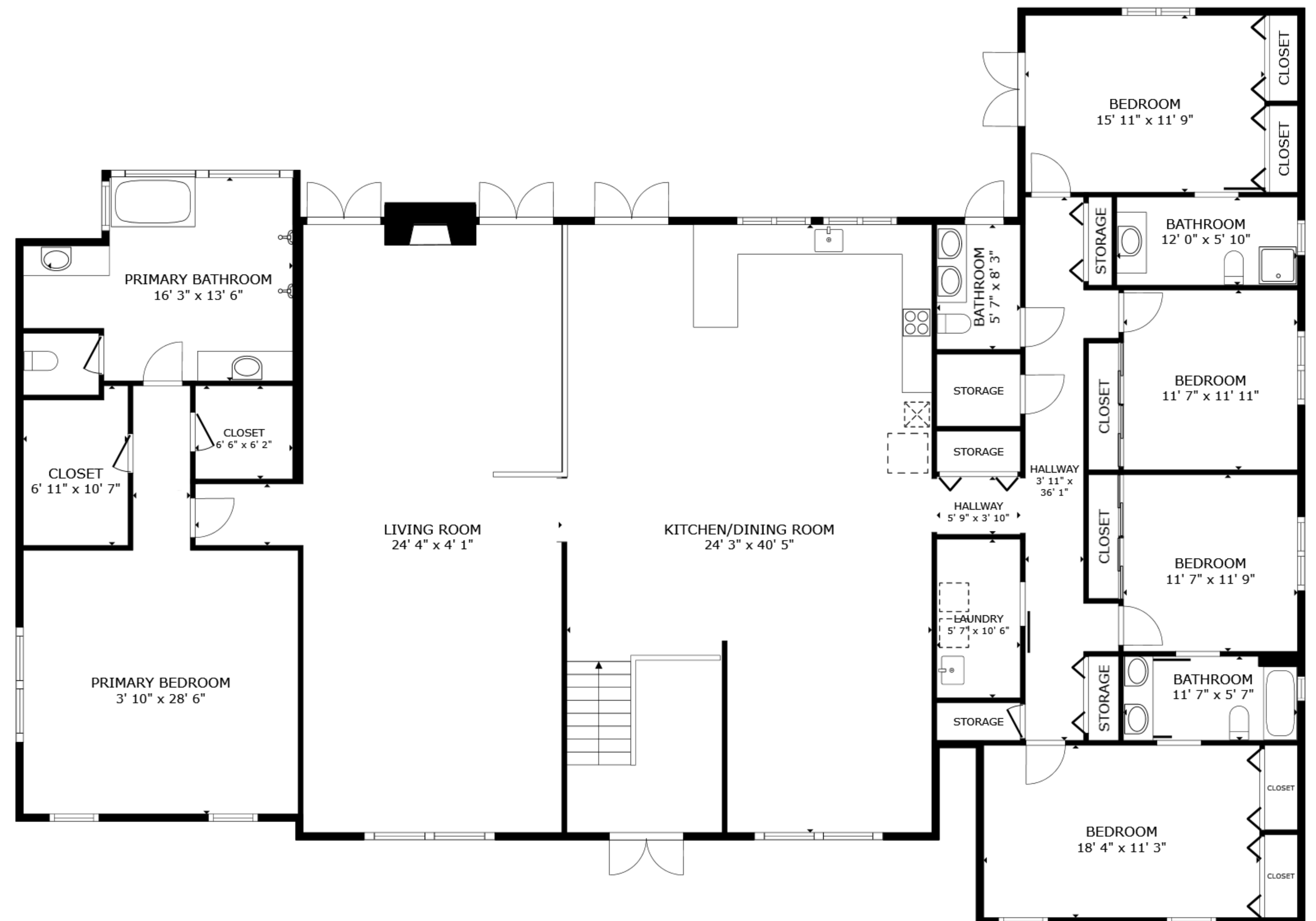
FLOOR 2
