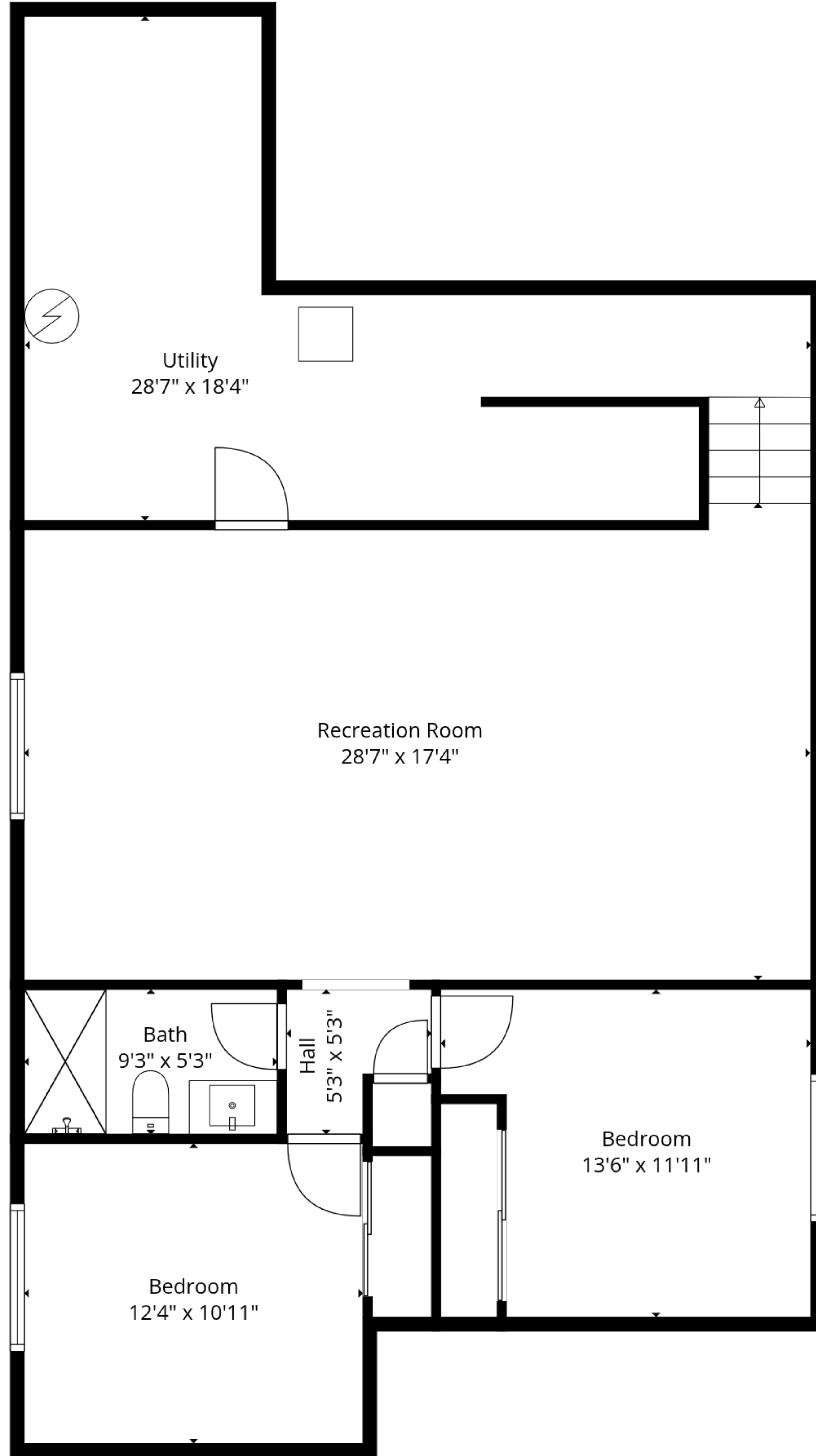
Basement 1
