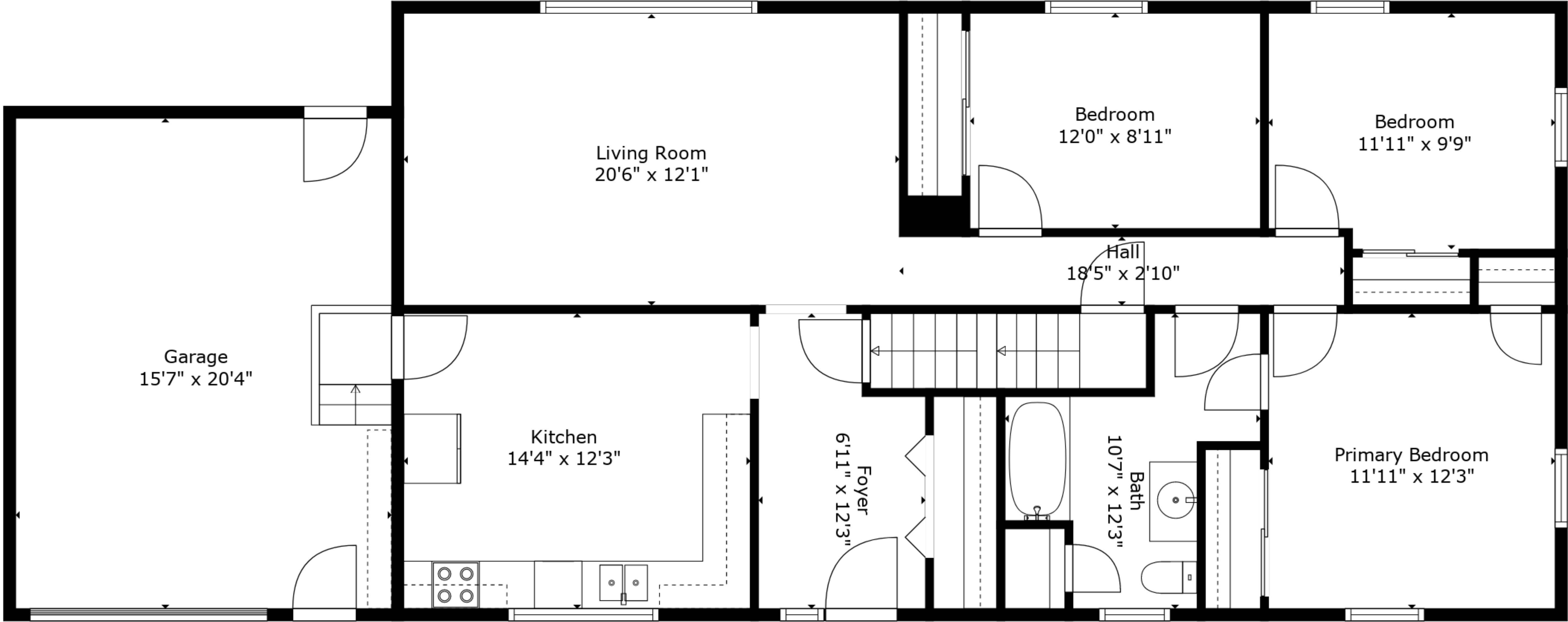
Floor 2
