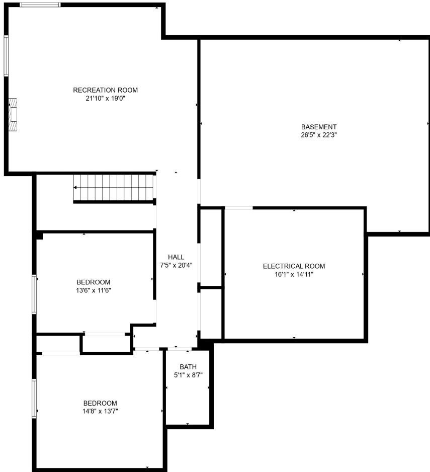
FLOOR 1
