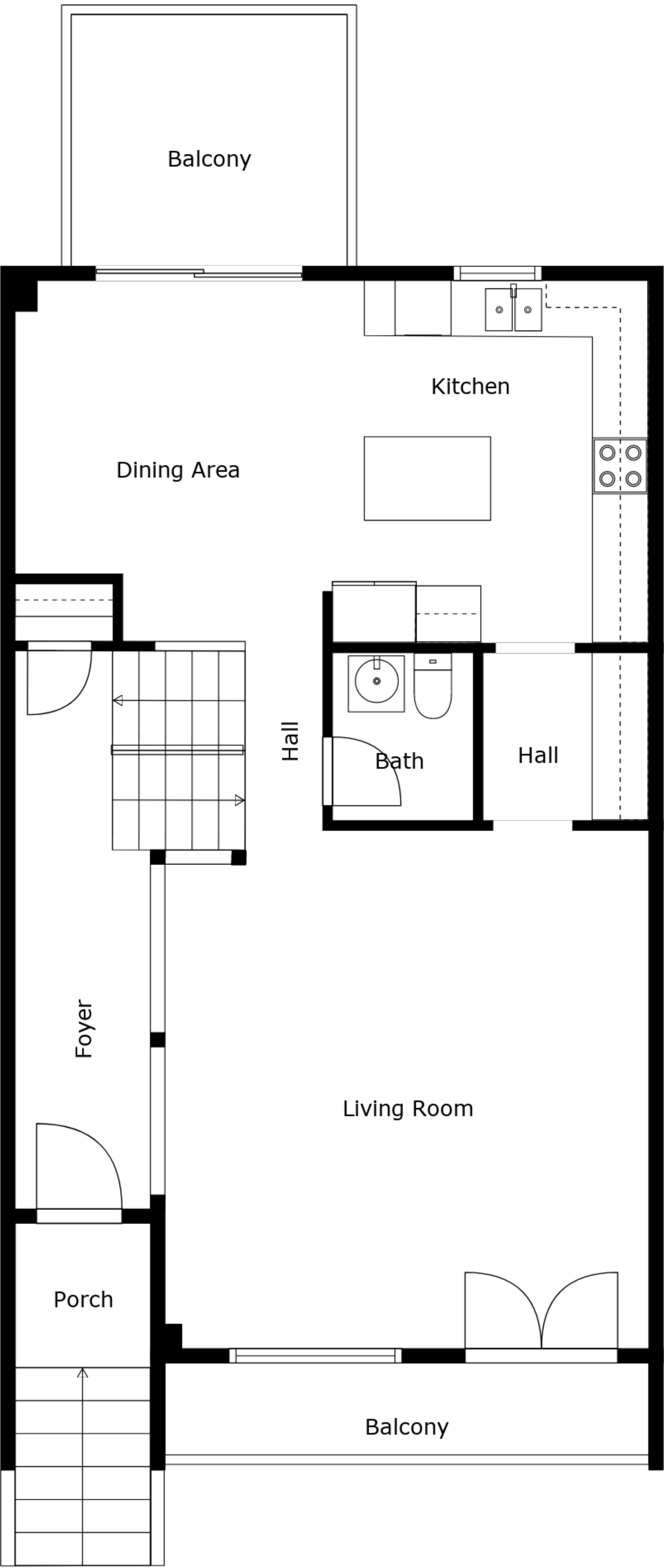
Floor 3
