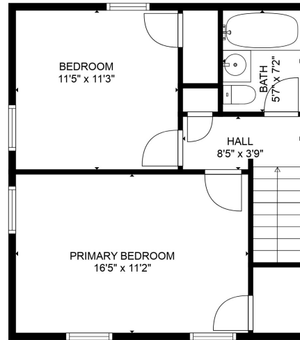
FLOOR 3
