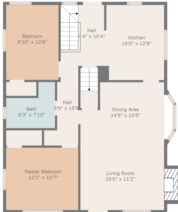
Floor 2
