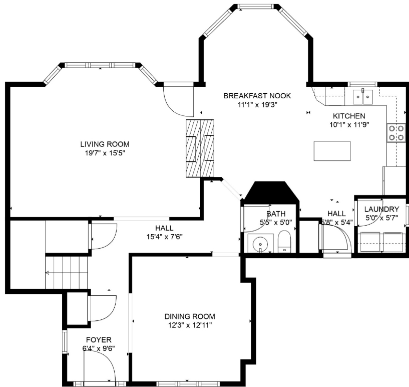
FLOOR 1
