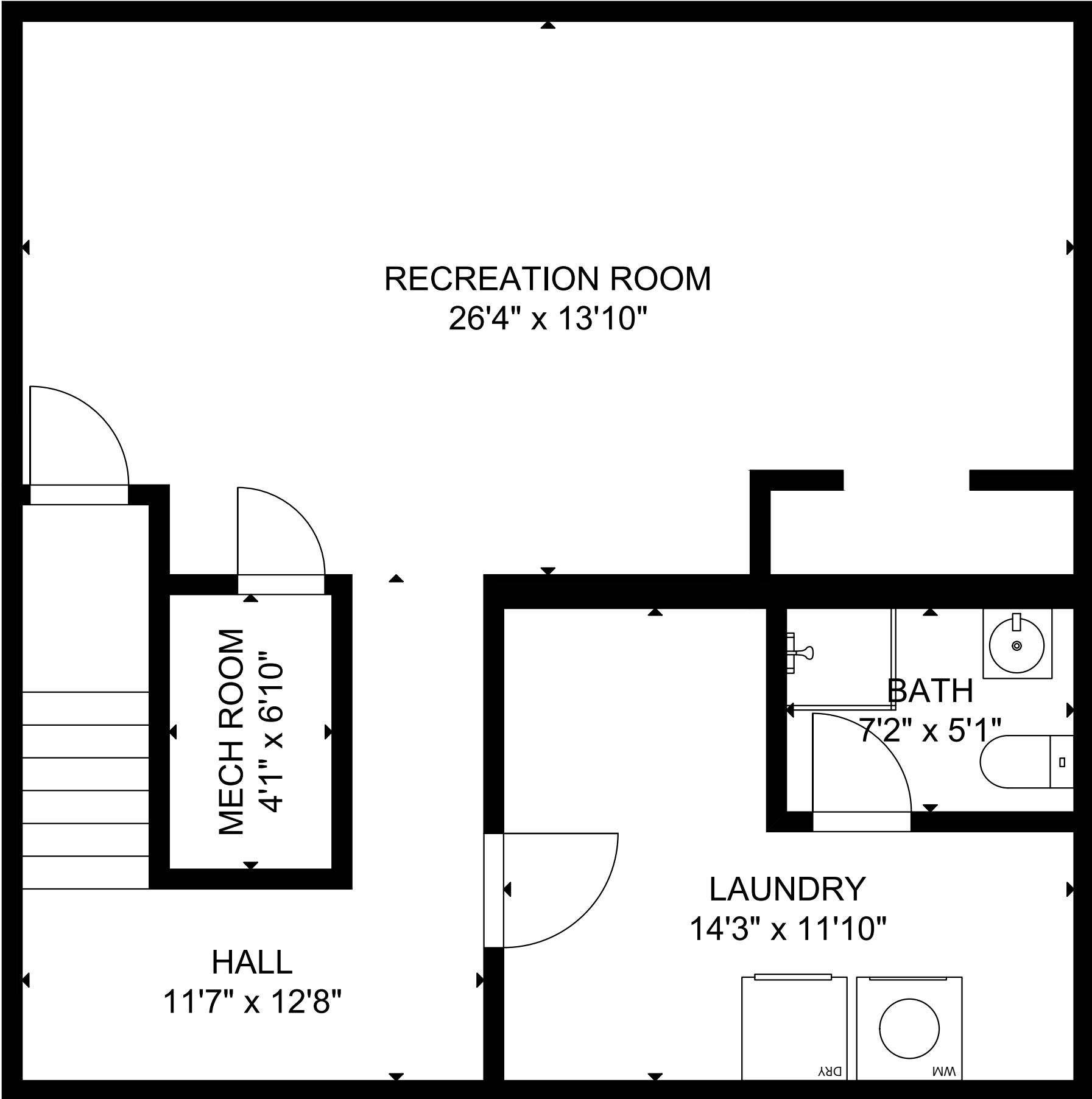
BASEMENT
