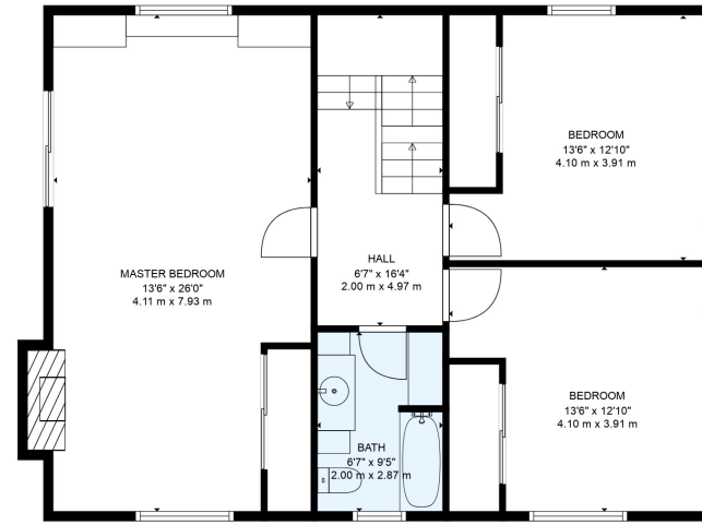
FLOOR 3
