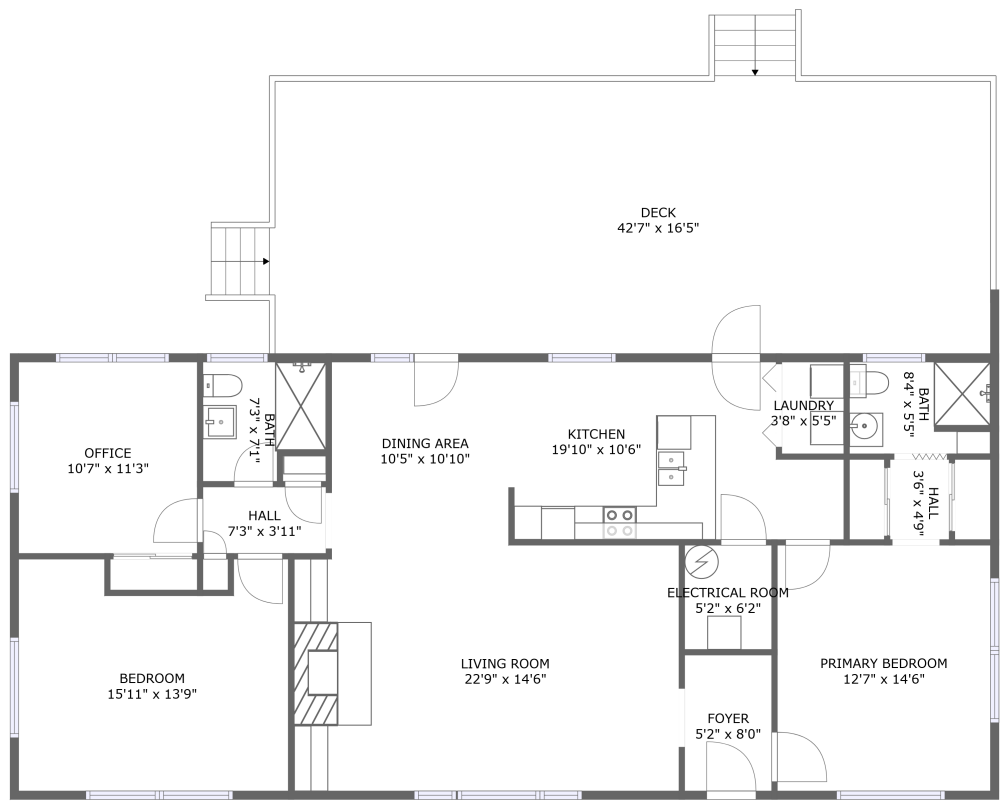
FLOOR 1
