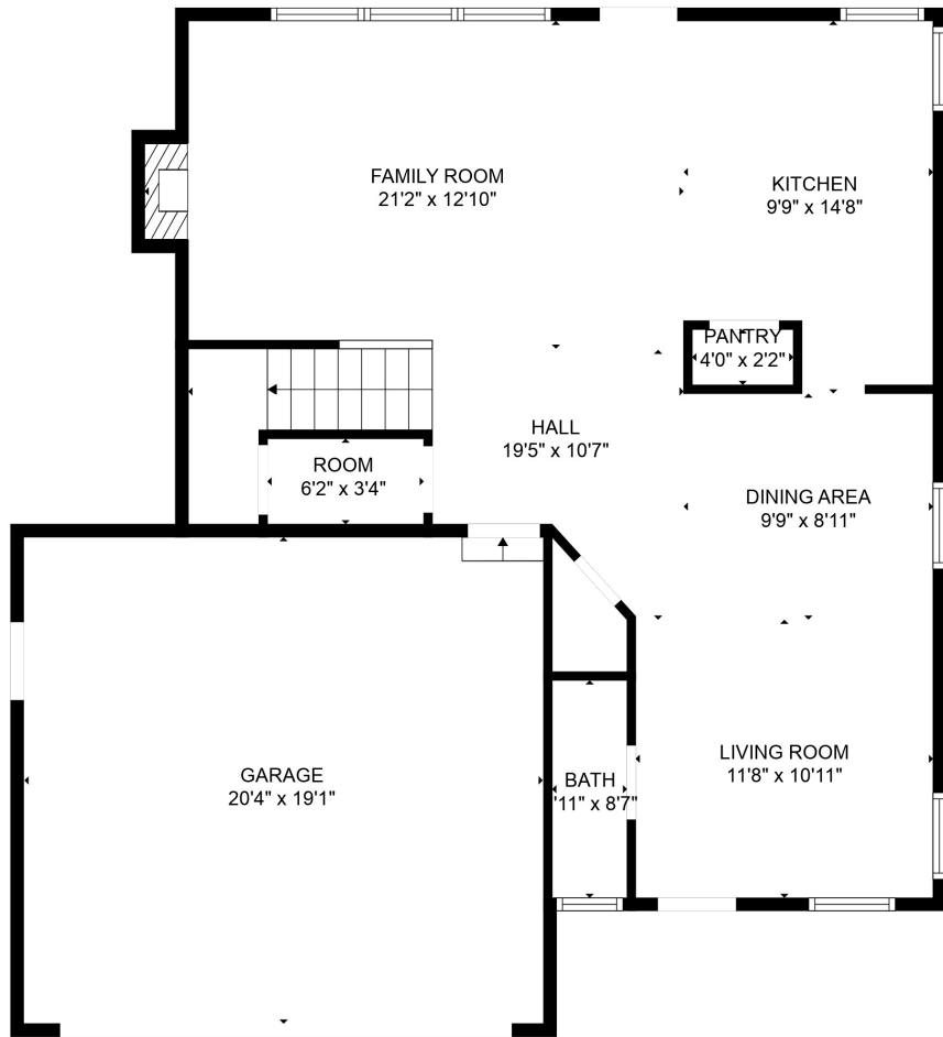
FLOOR 1
