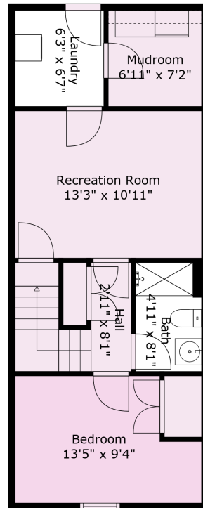
Floor 1
