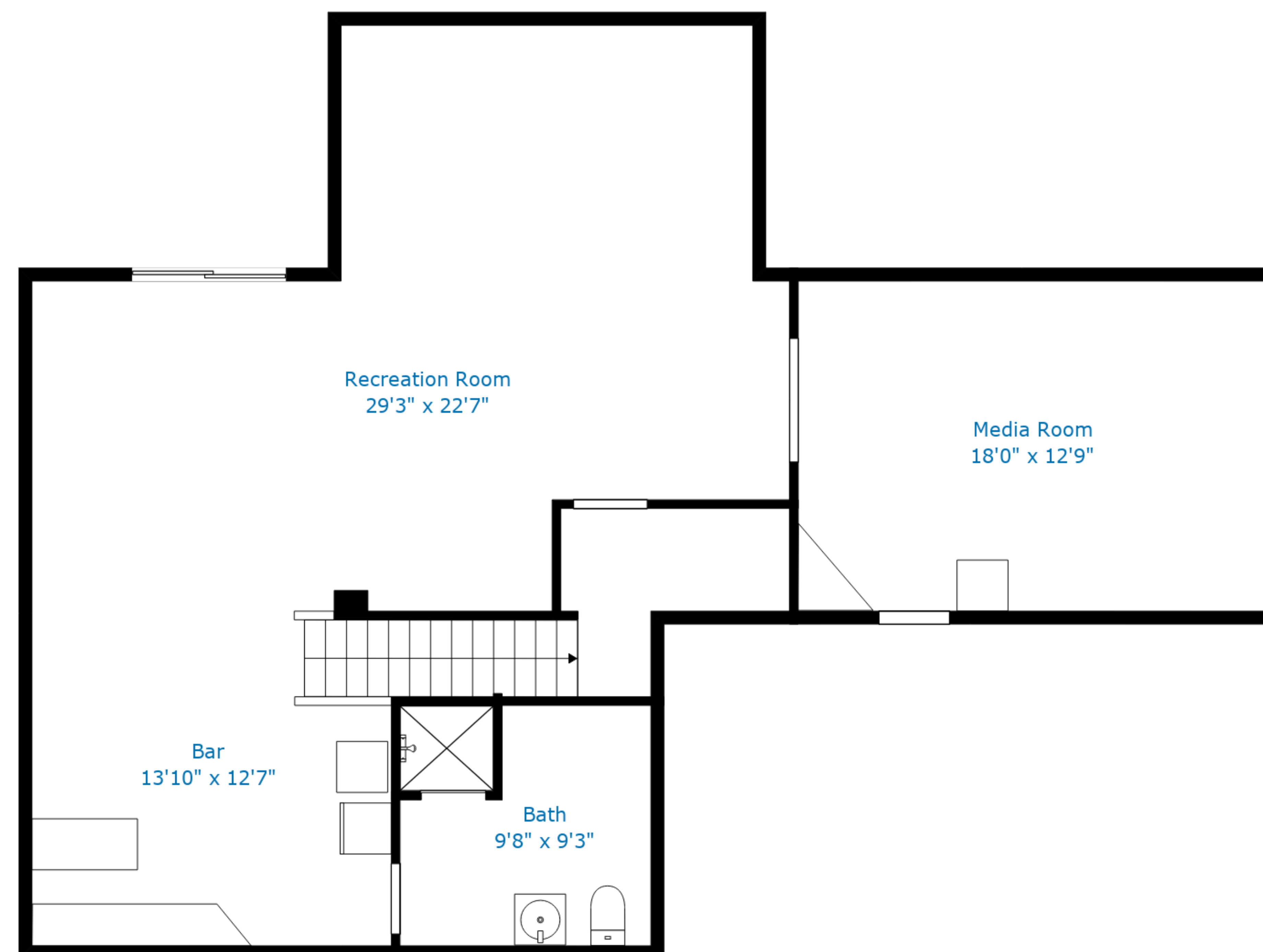
Floor 1
