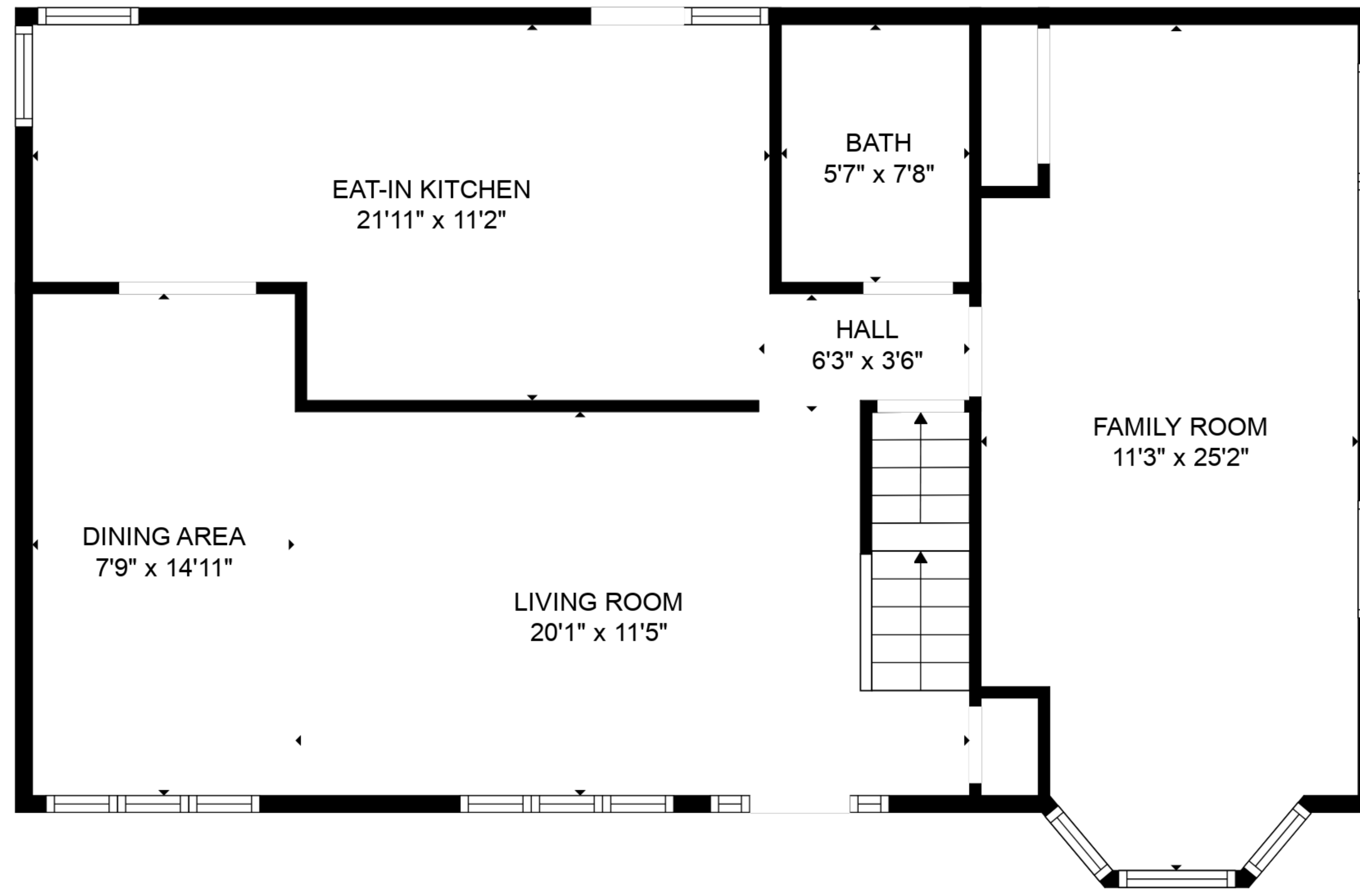
FLOOR 2
