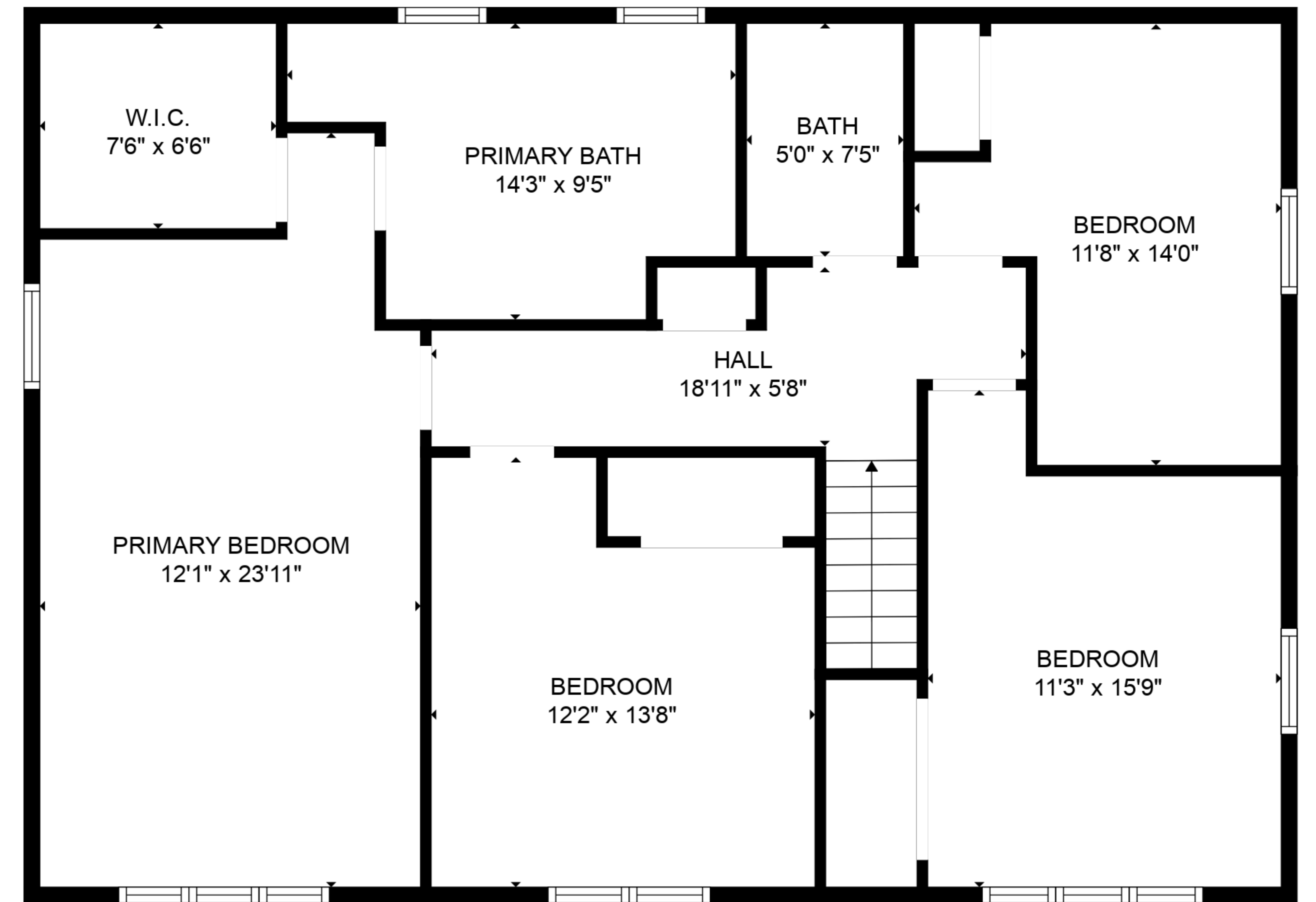
FLOOR 3
