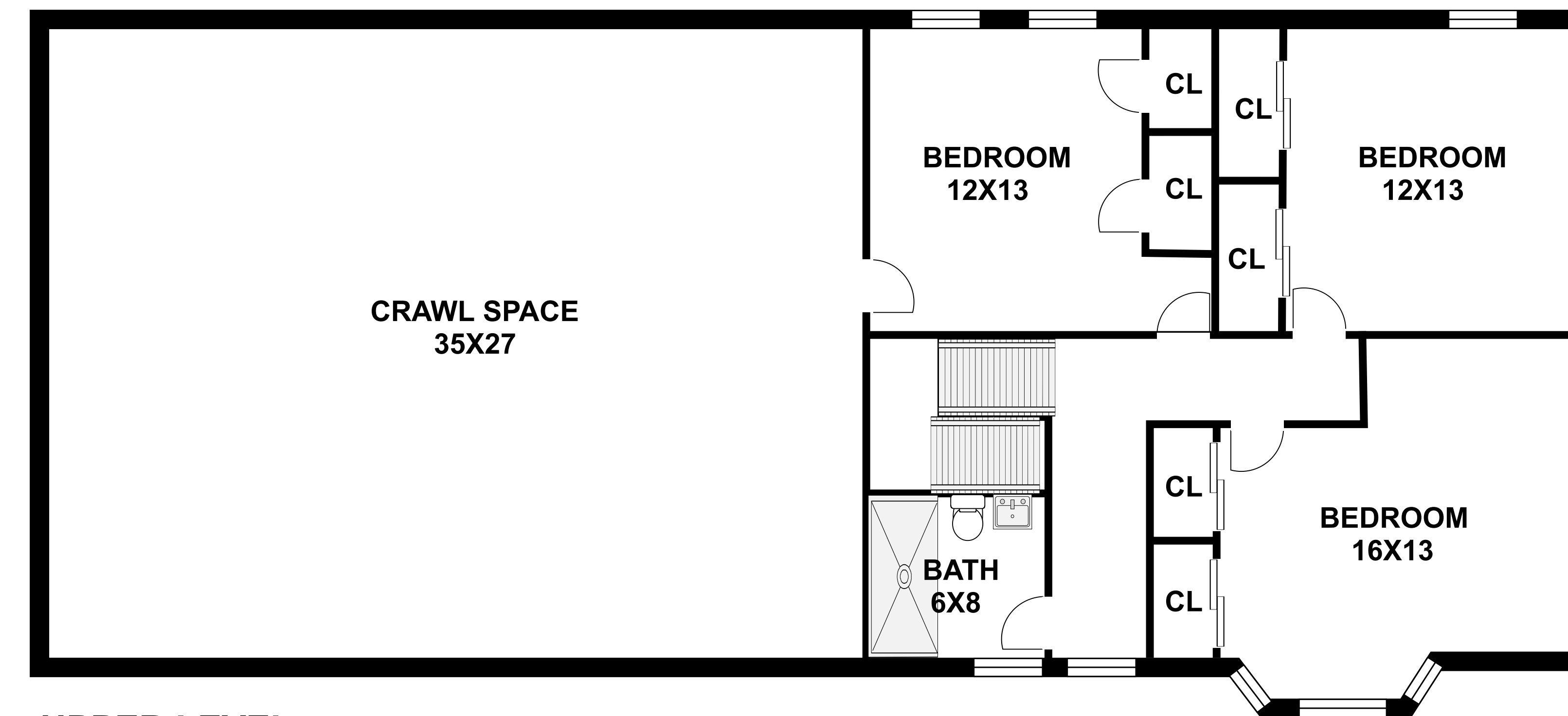
UPPER LEVEL
