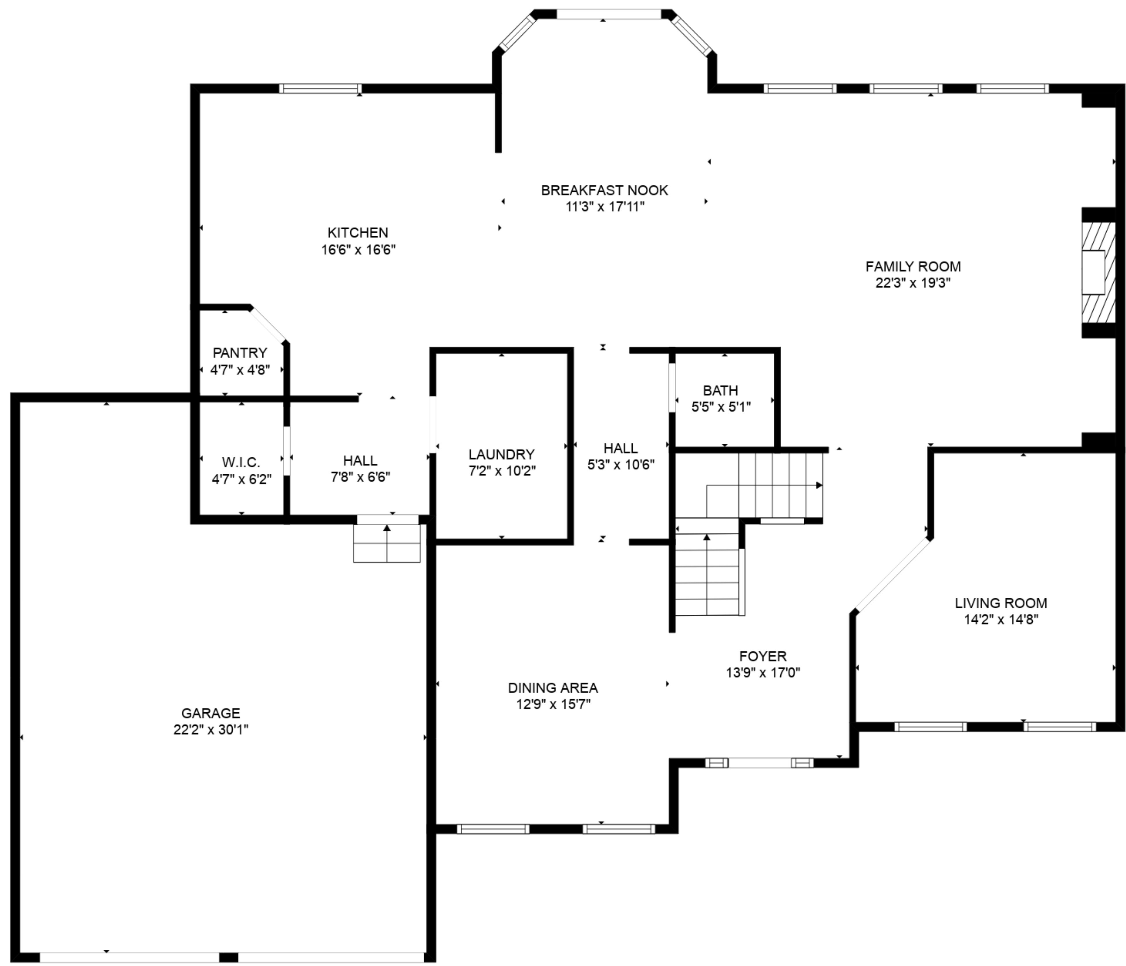
FLOOR 2
