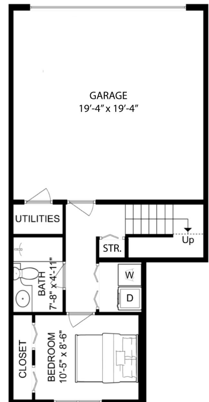
LOWER FLOOR 335 sq.ft. | Ceiling Height: 8'-0"
