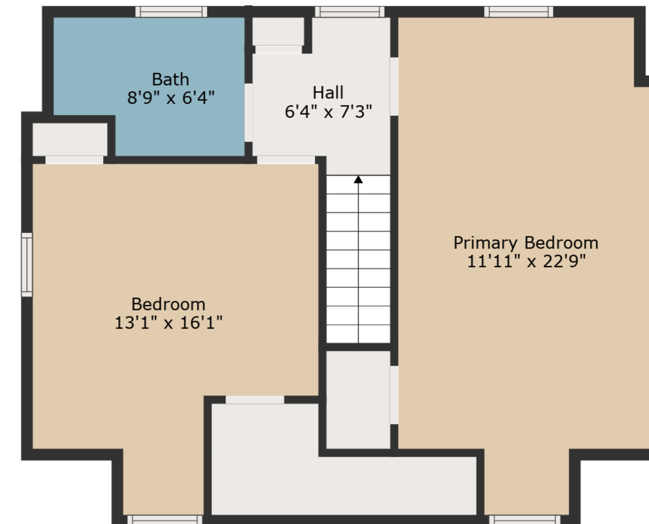
Floor 3
