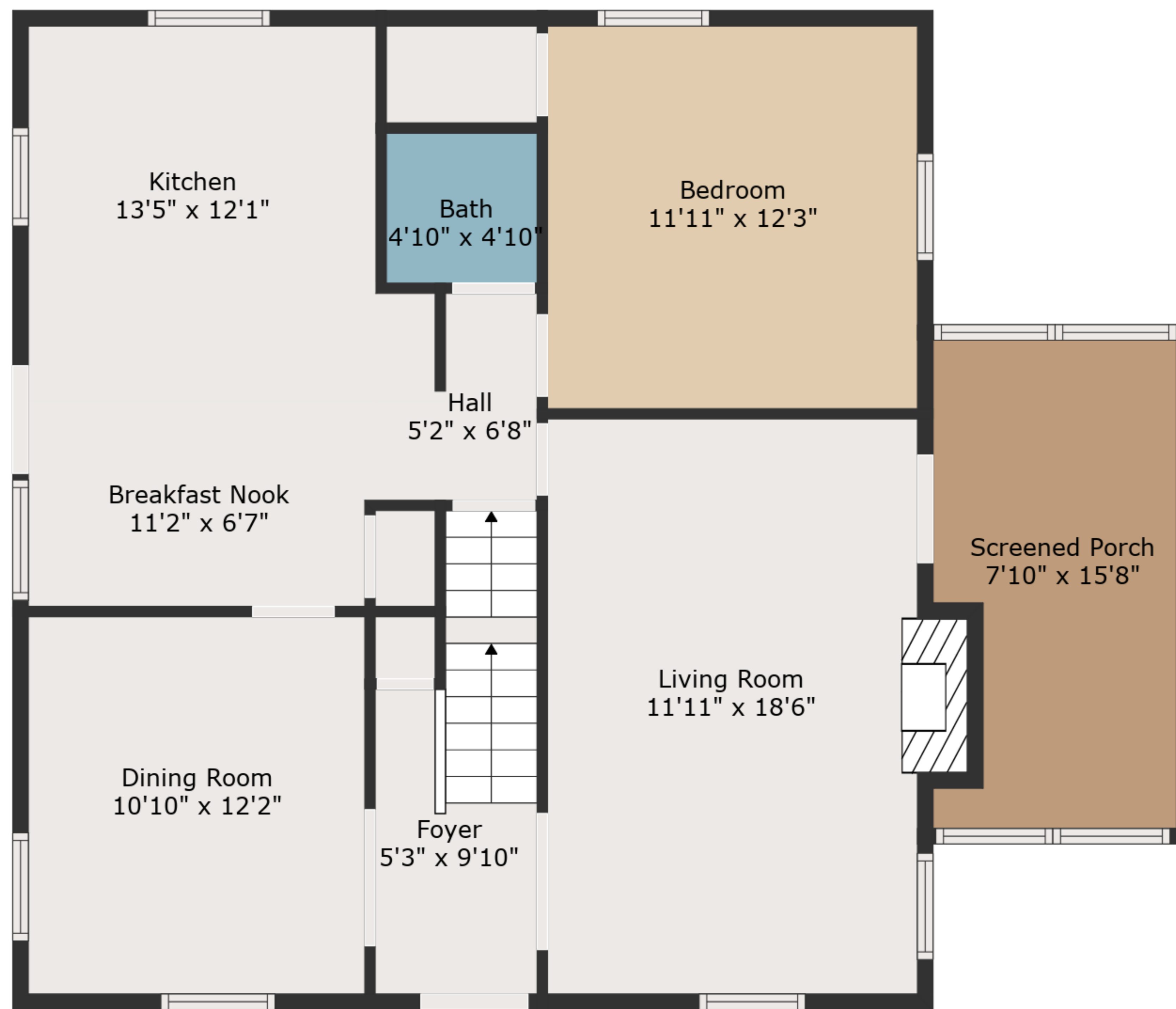
Floor 2
