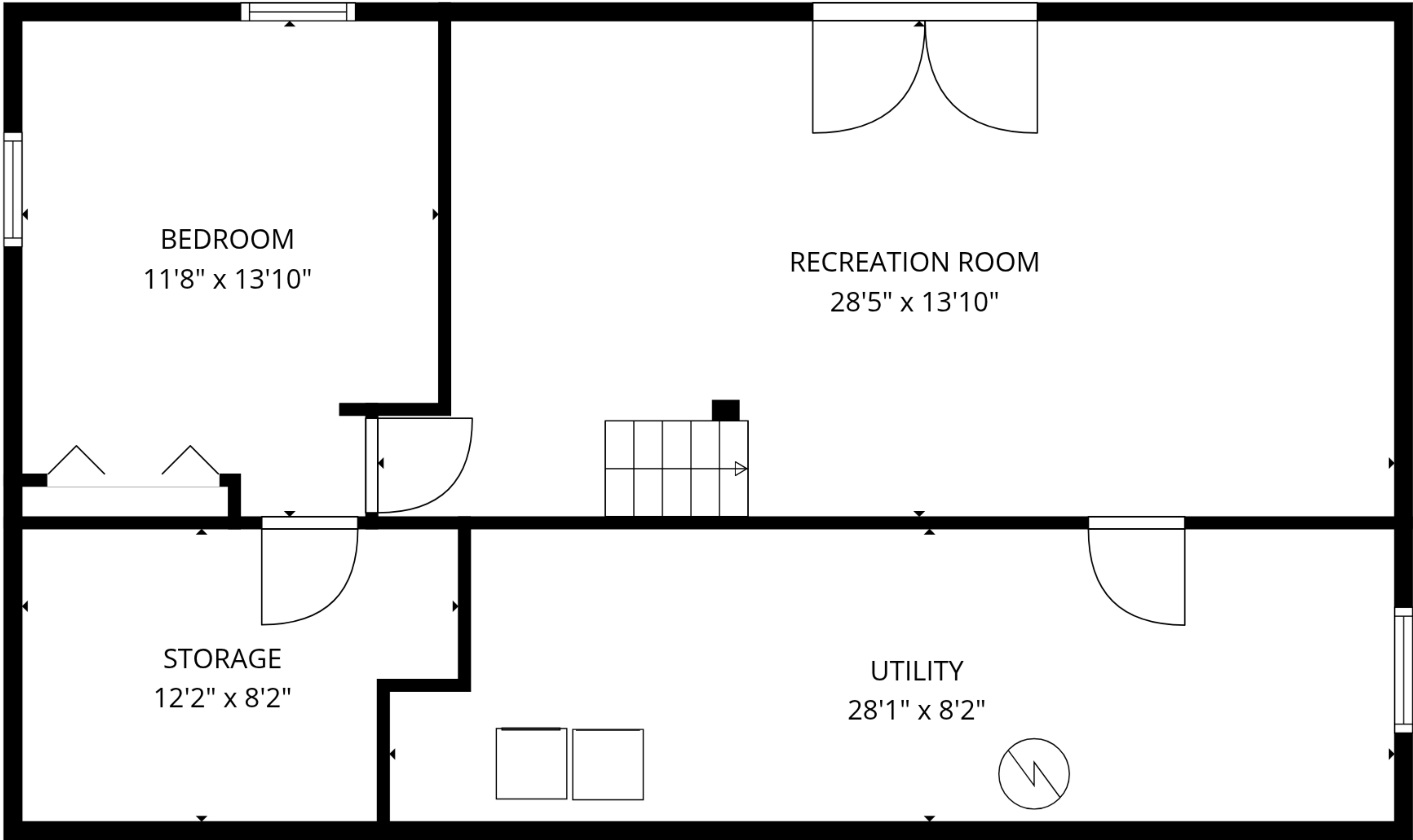
FLOOR 2
