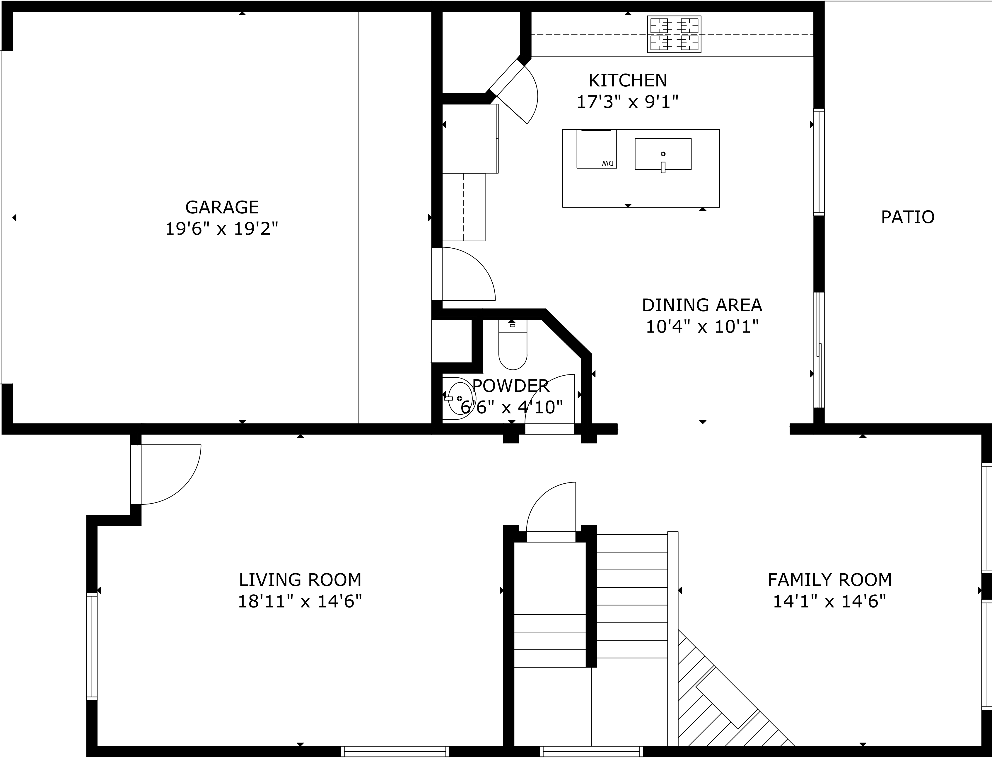
FLOOR 1
