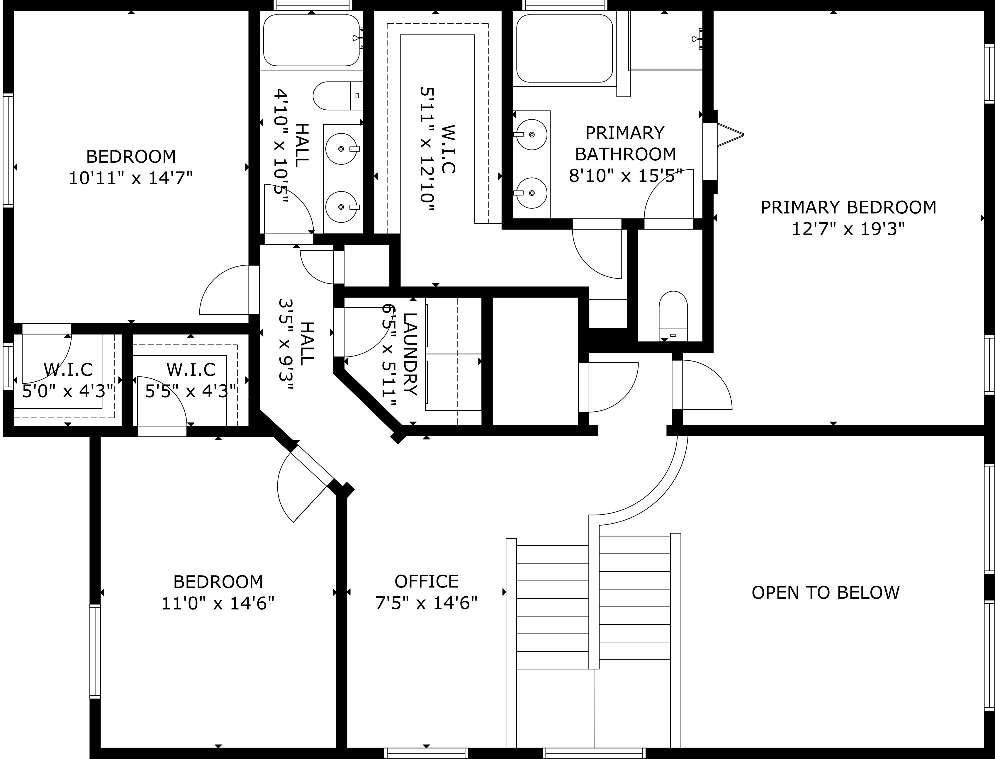
FLOOR 2
