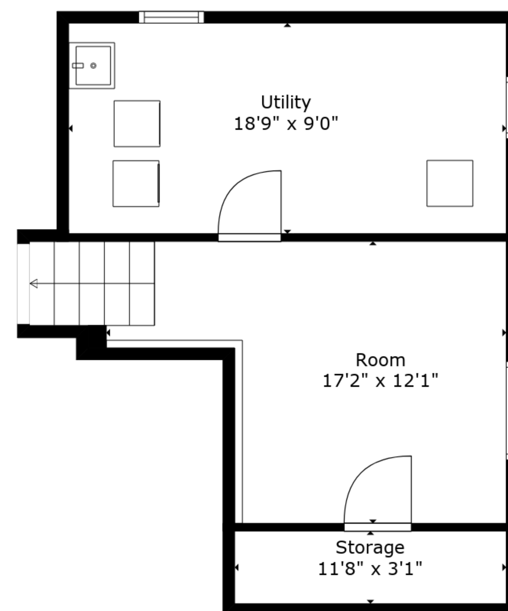
Floor 1
