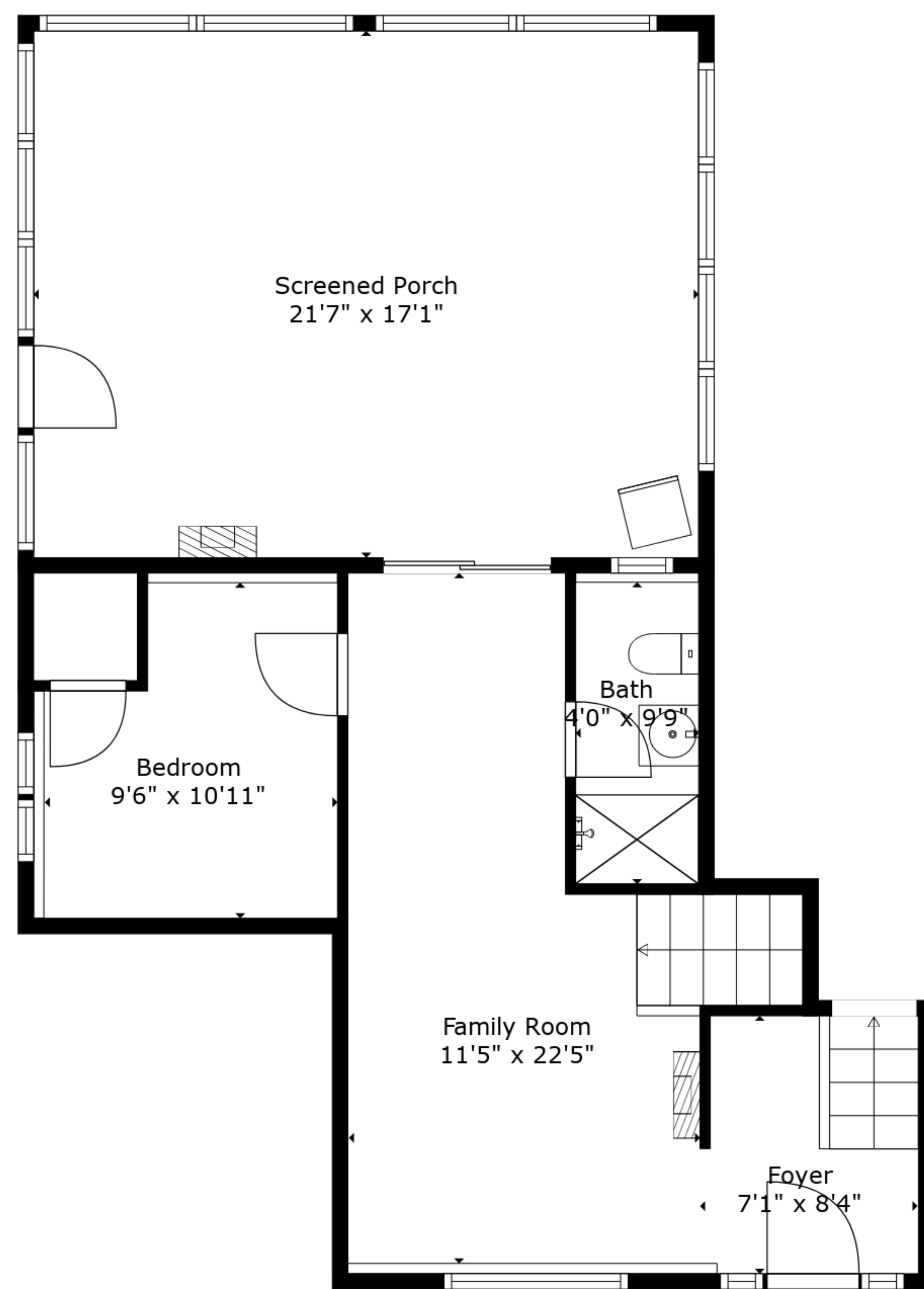
Floor 2
