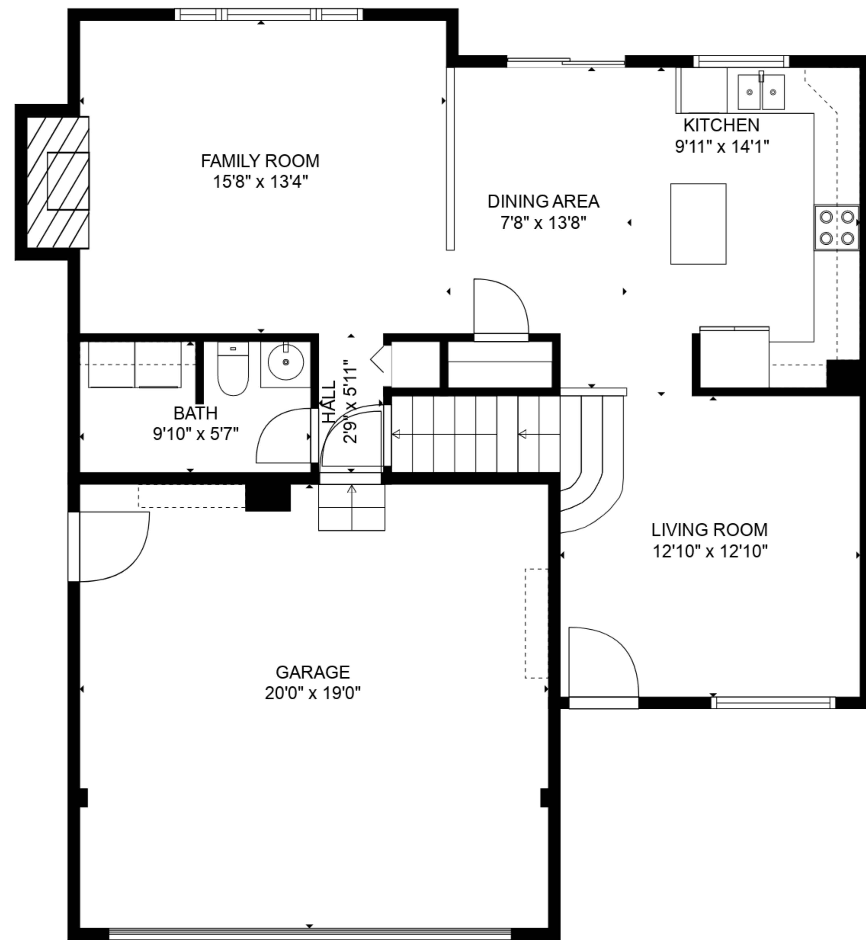
FLOOR 2
