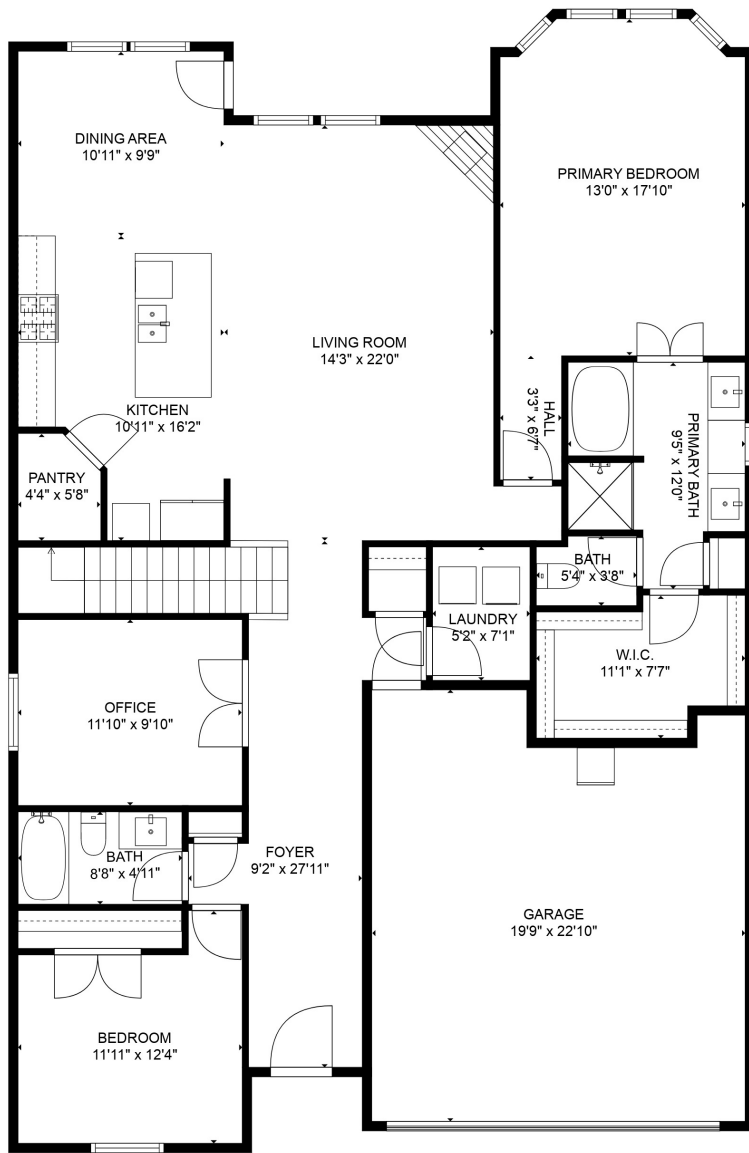
FLOOR 1
