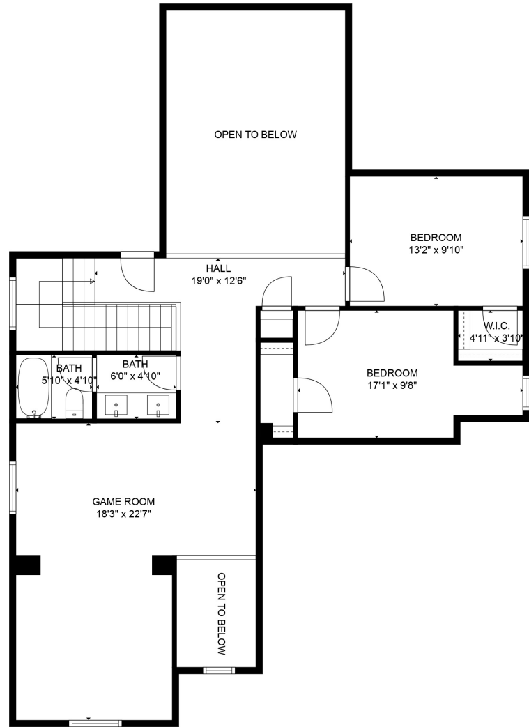
FLOOR 2
