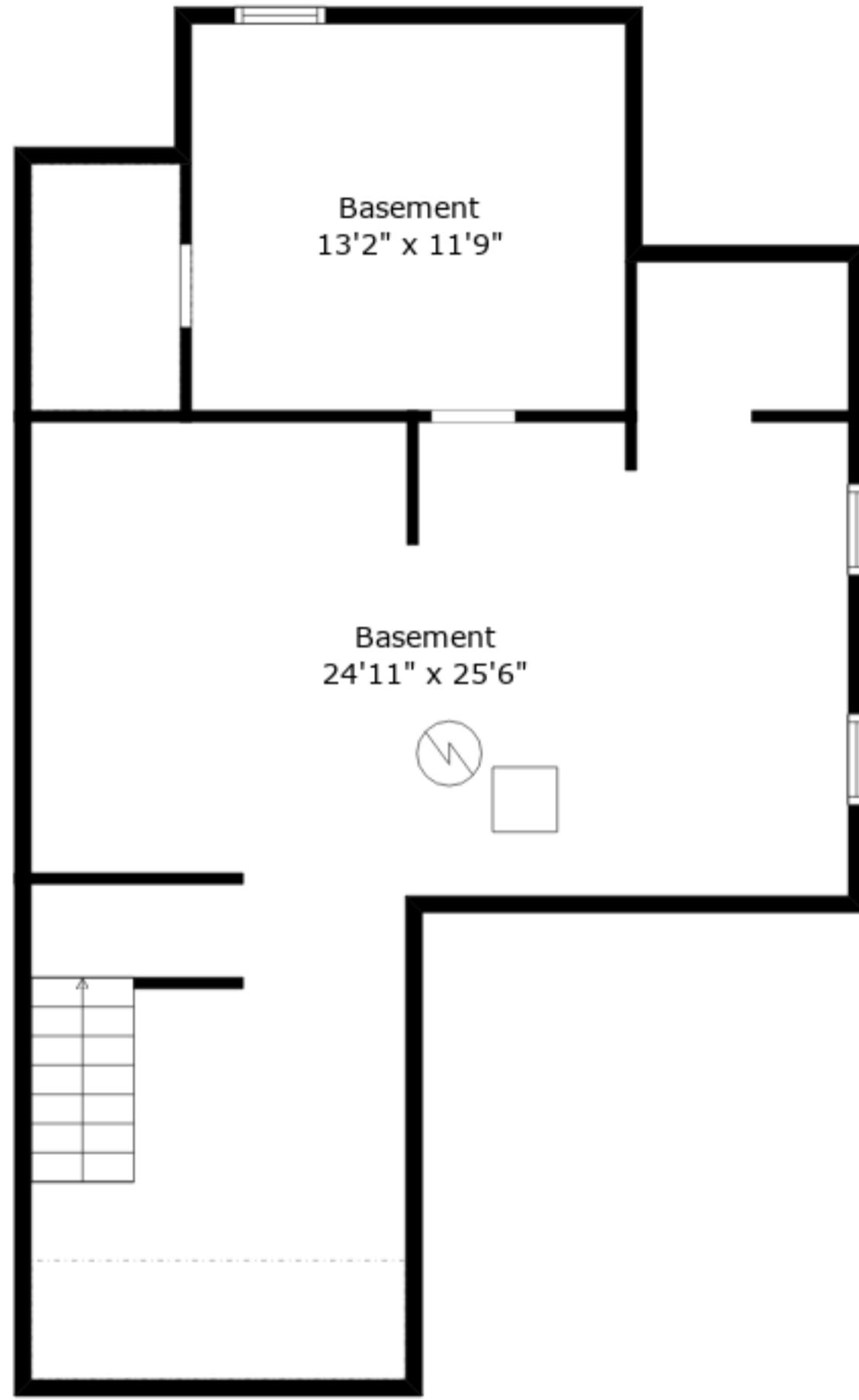
Lower Floor
