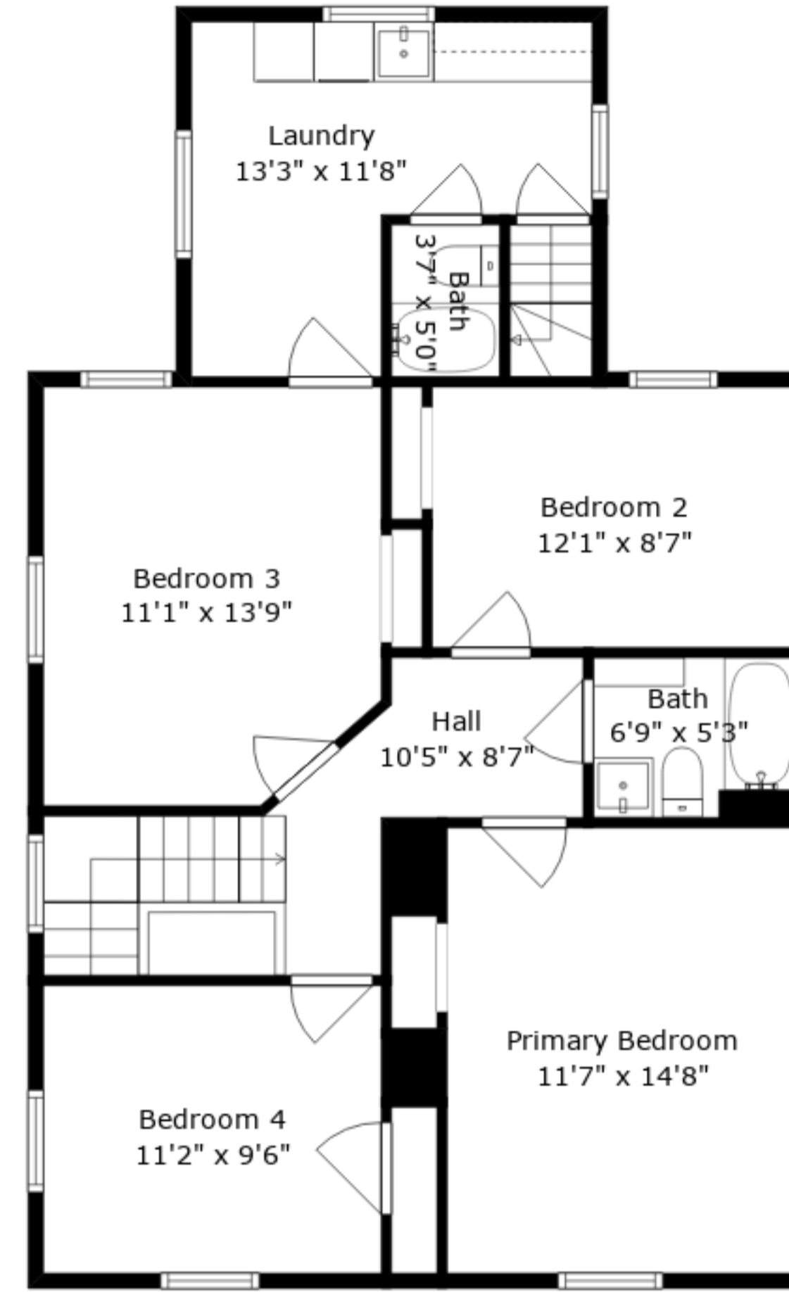
Upper Floor
