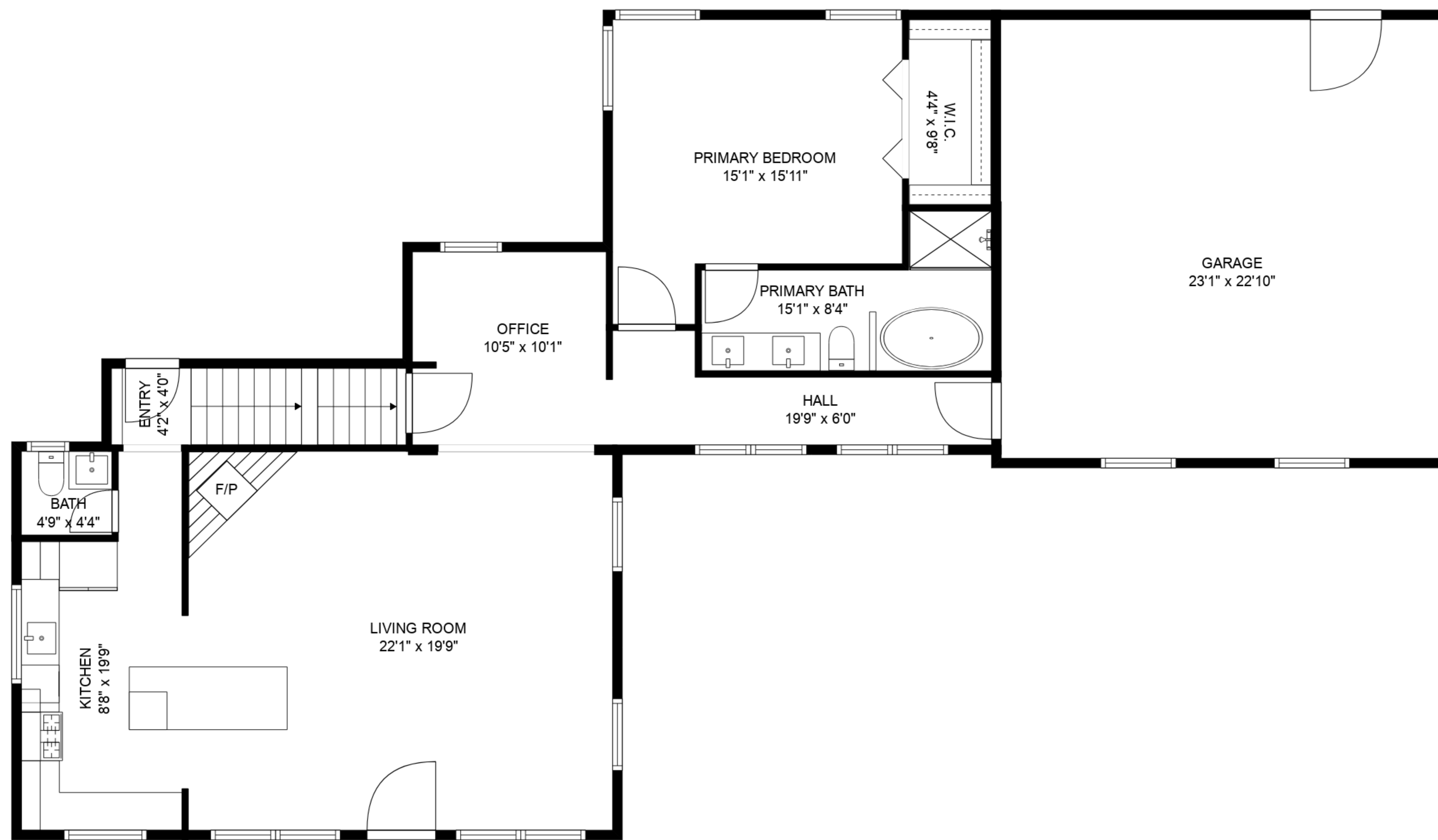
FLOOR 2
