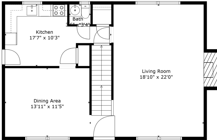
Floor 2
