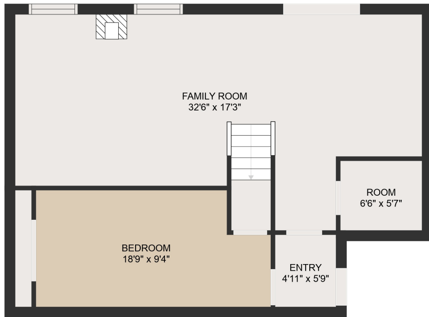
FLOOR 1
