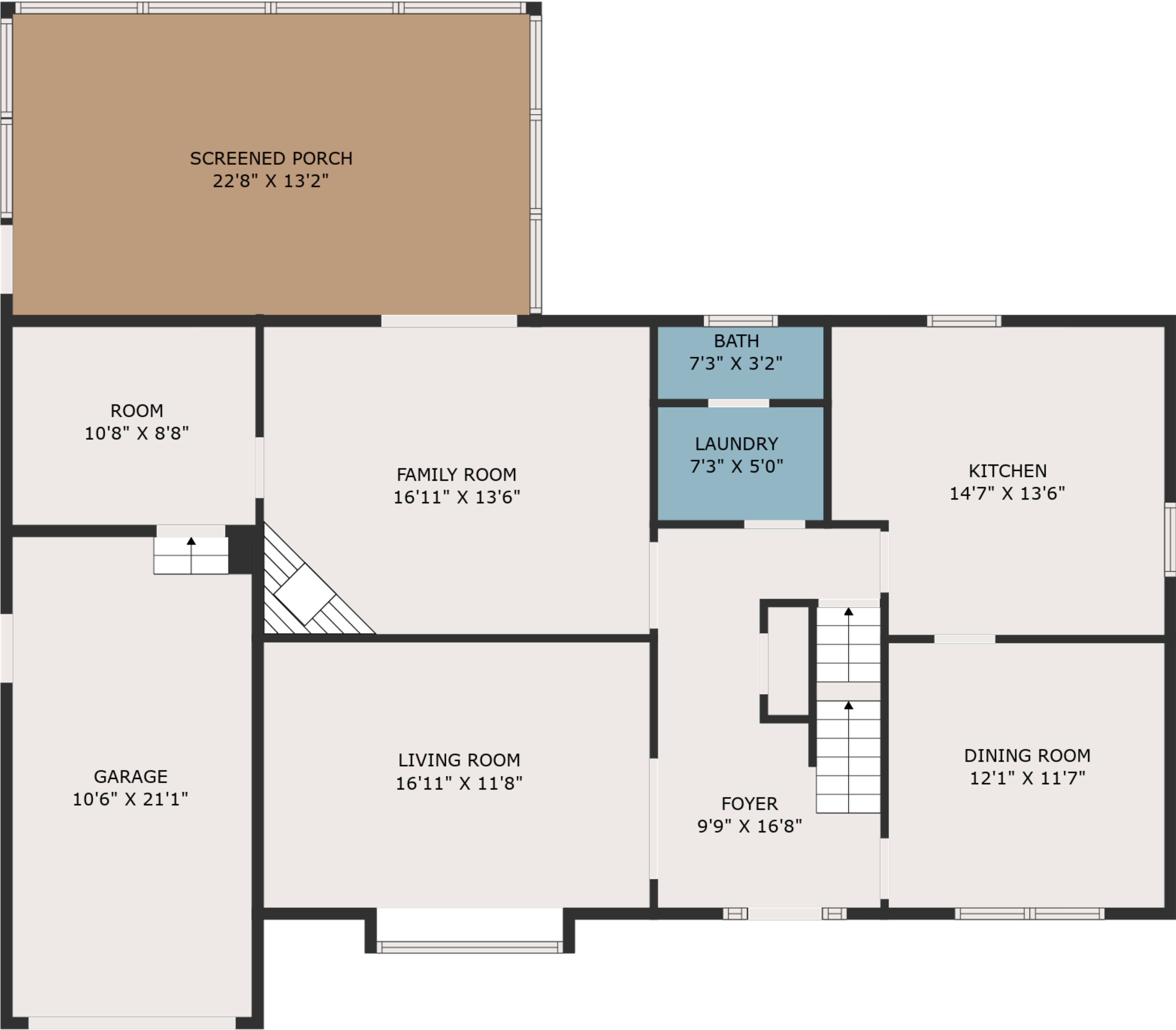
FLOOR 2
