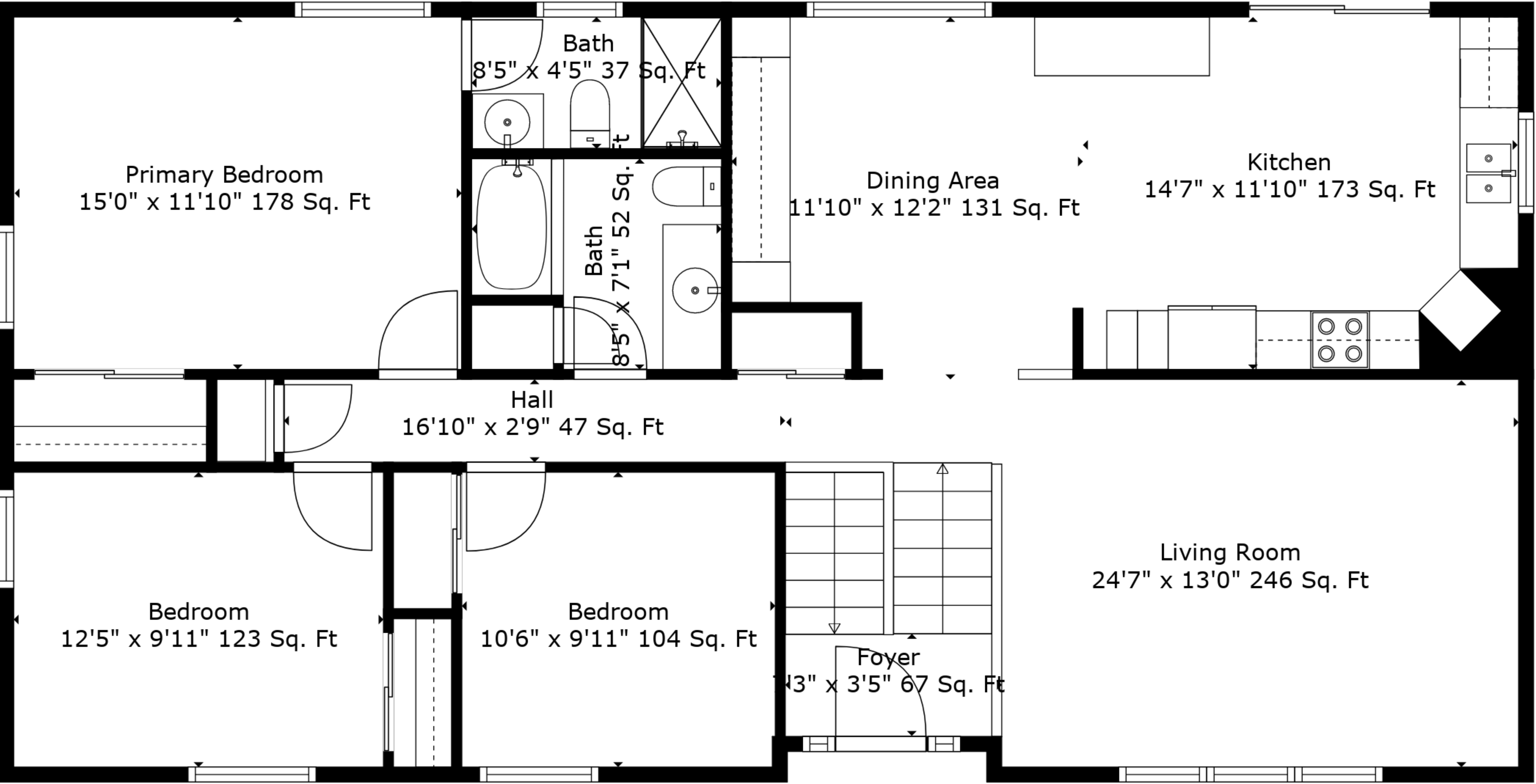
Floor 2
