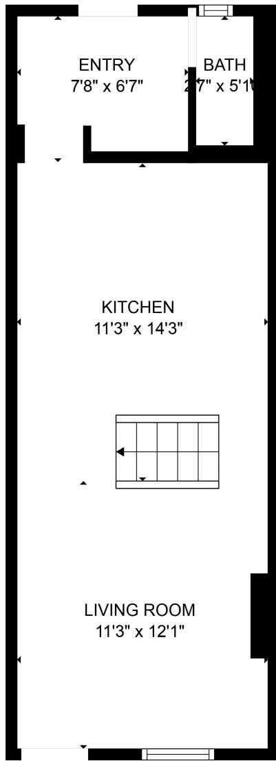
FLOOR 1
