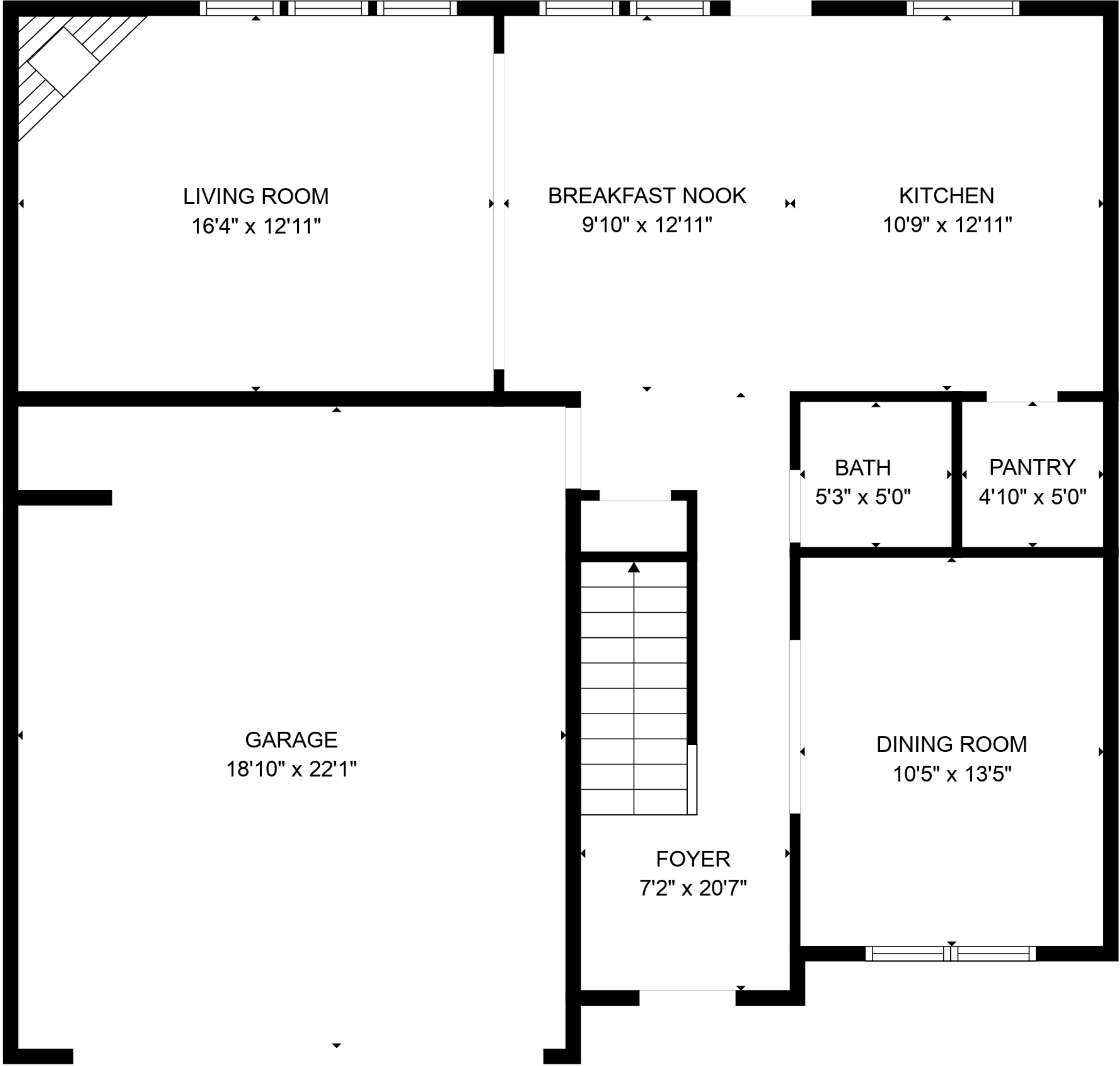
FLOOR 1
