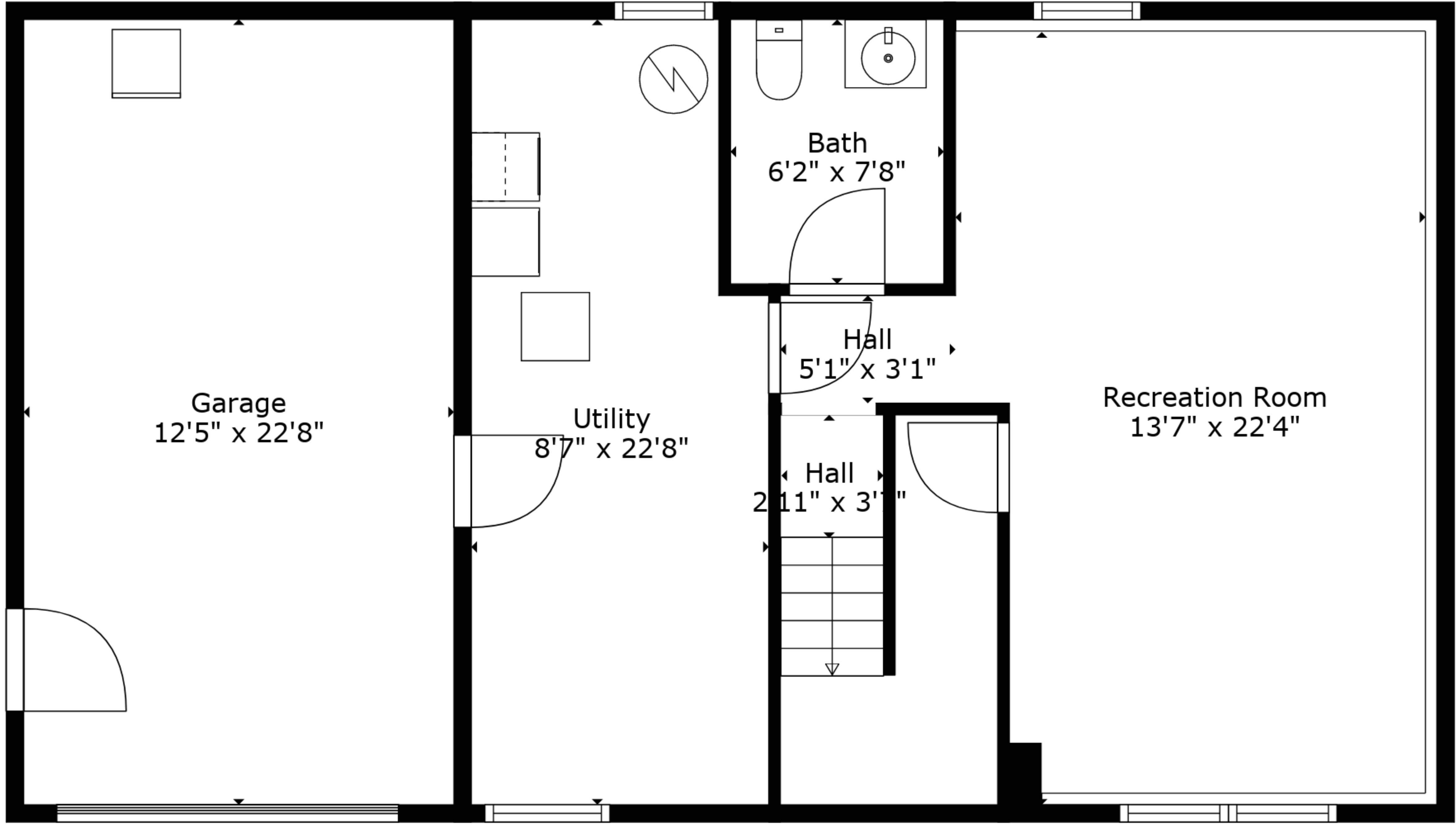
Floor 2
